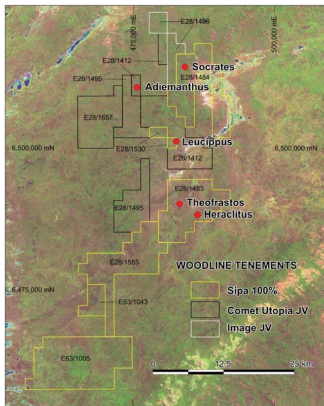
Figure 7 - Woodline Gold Project on Landsat Image.
