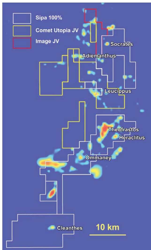
Figure 8 - Woodline - Gold in-Calcrete Image & Prospects
