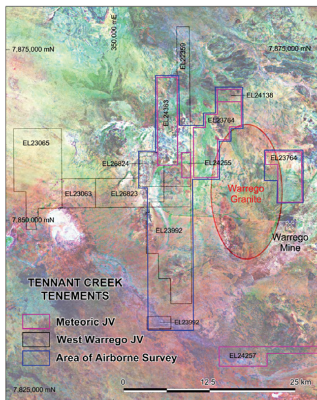
Figure 10 - Tennant Creek Gold-Copper Projects on Landsat Image.
