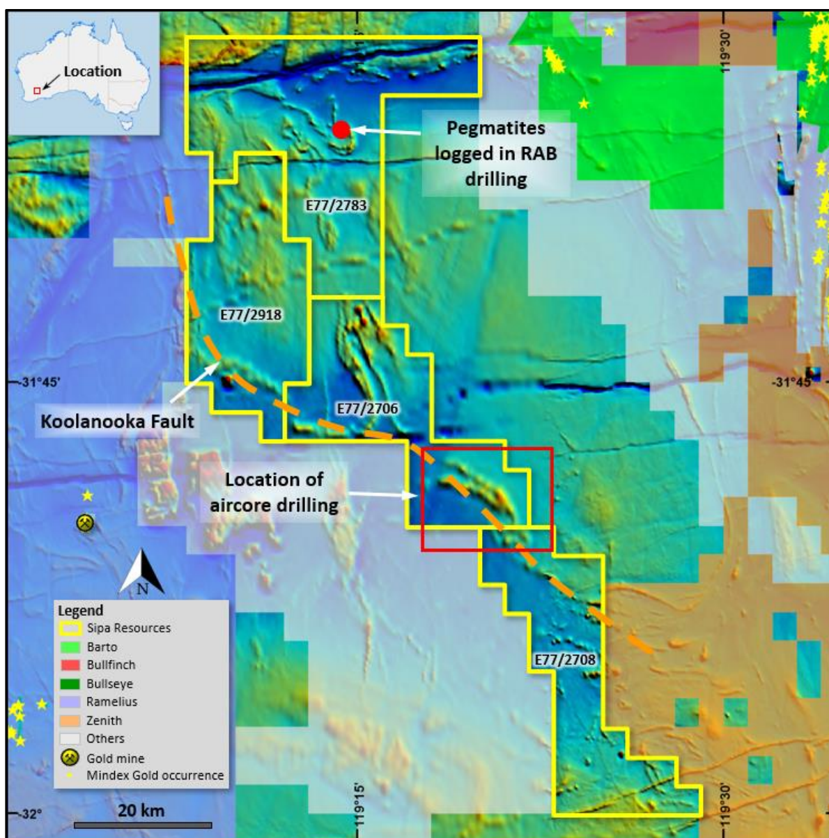
Figure 1: Skeleton Rocks Project showing the location of aircore drilling completed earlier in 2022.
