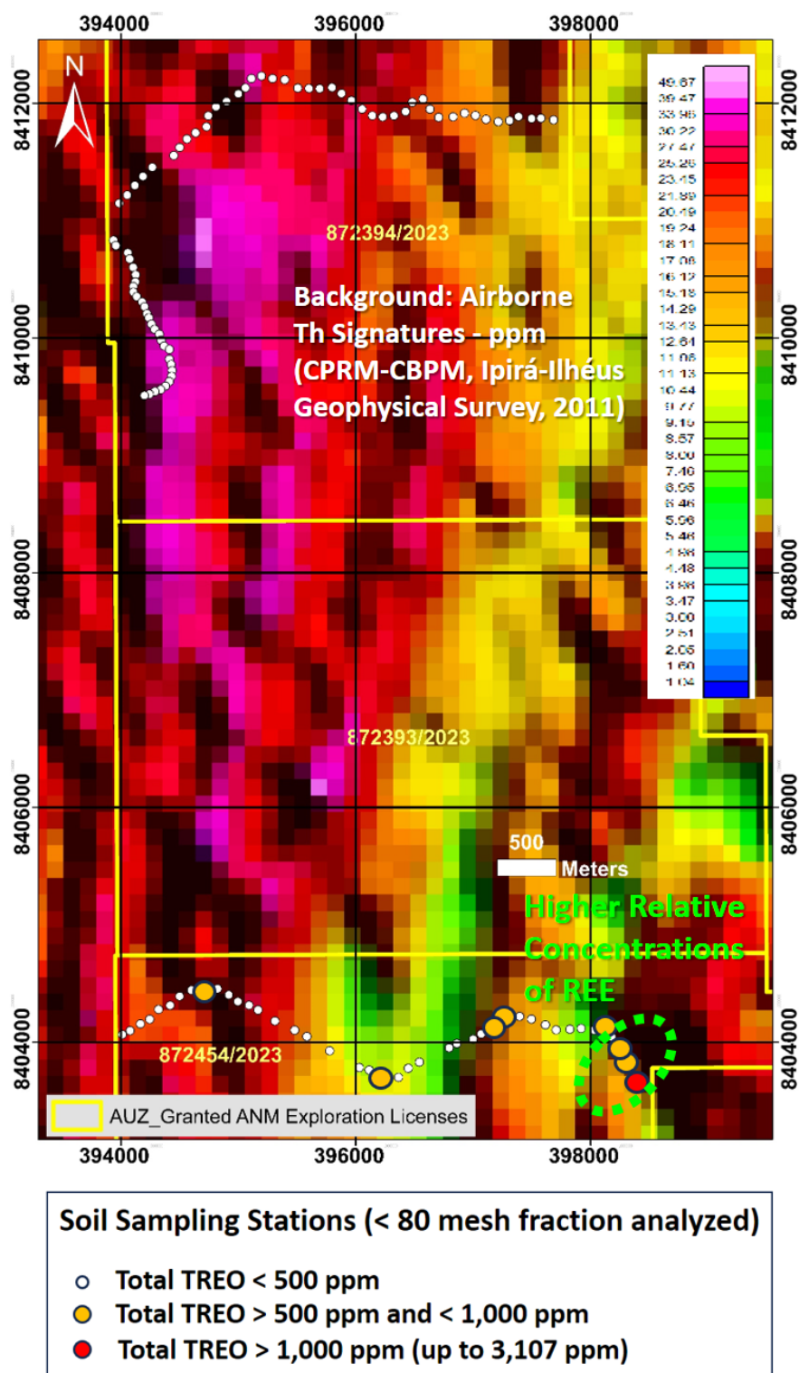
Figure 2: Jequie South Target. The green encircled area indicates the potential presence of new type of REE mineralization.
