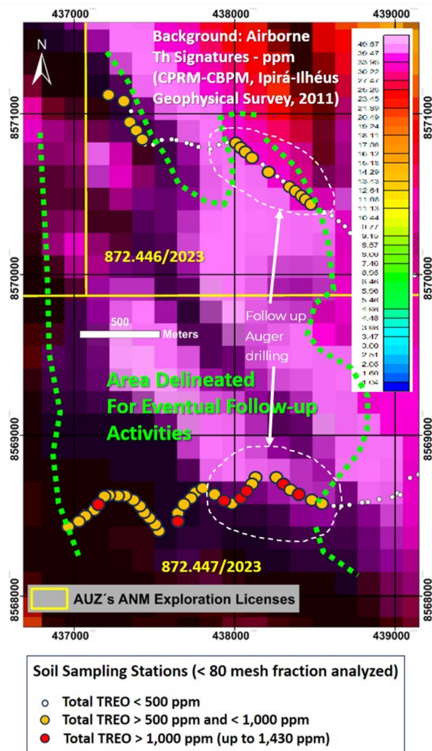
Figure 1: Jeiquie North Target
