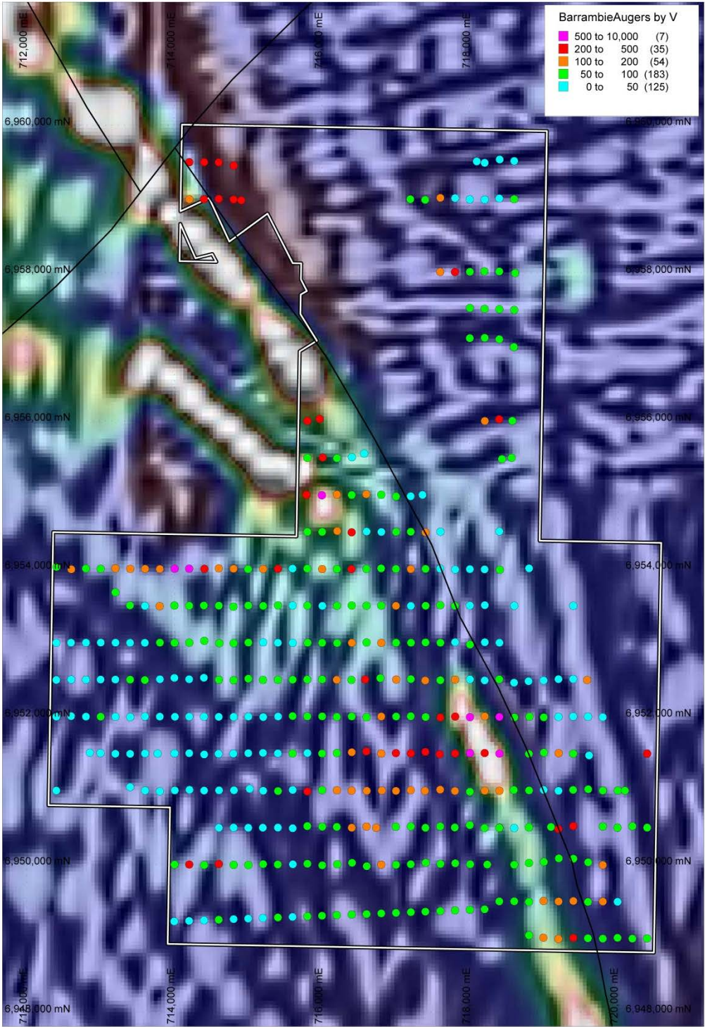
Figure 2: Auger Samples: Thematically Mapped: Vanadium Values (ppm) on Magnetic Image
