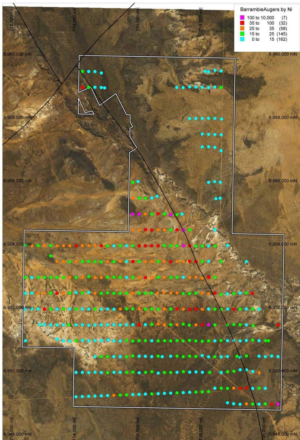
Figure 3: Auger Samples: Thematically Mapped: Nickel Values (ppm)
