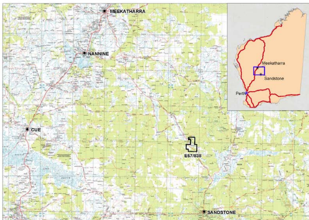
Figure 1: Regional Location Plan: E57/838
