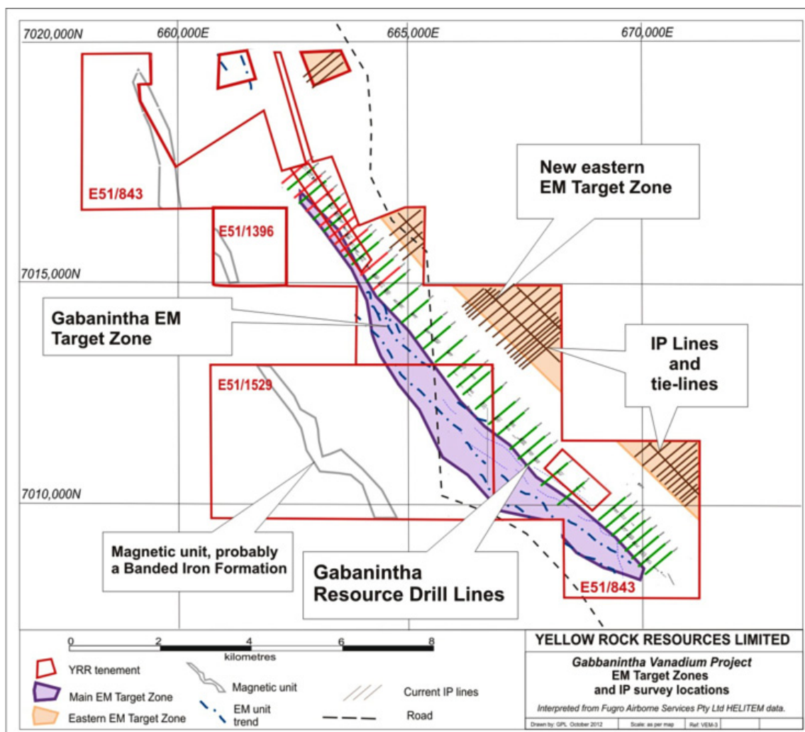
Figure 1 - Plan showing new eastern EM target zone and IP survey locations.
