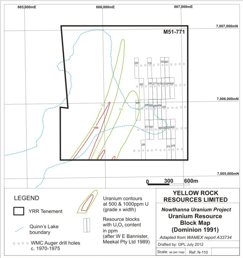
Figure 2: Dominion Resource Blocks and grade contours in 1991
