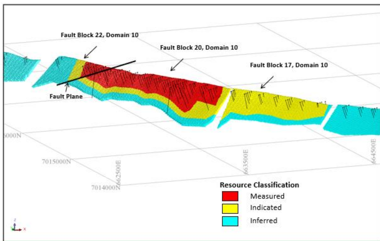
Figure 6 Resource Classification Gabanintha Deposit
