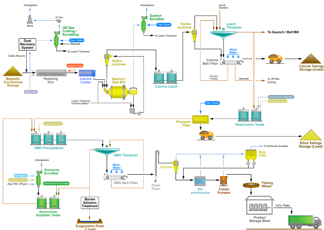
Figure 16 Refinery Flowsheet Schematic
