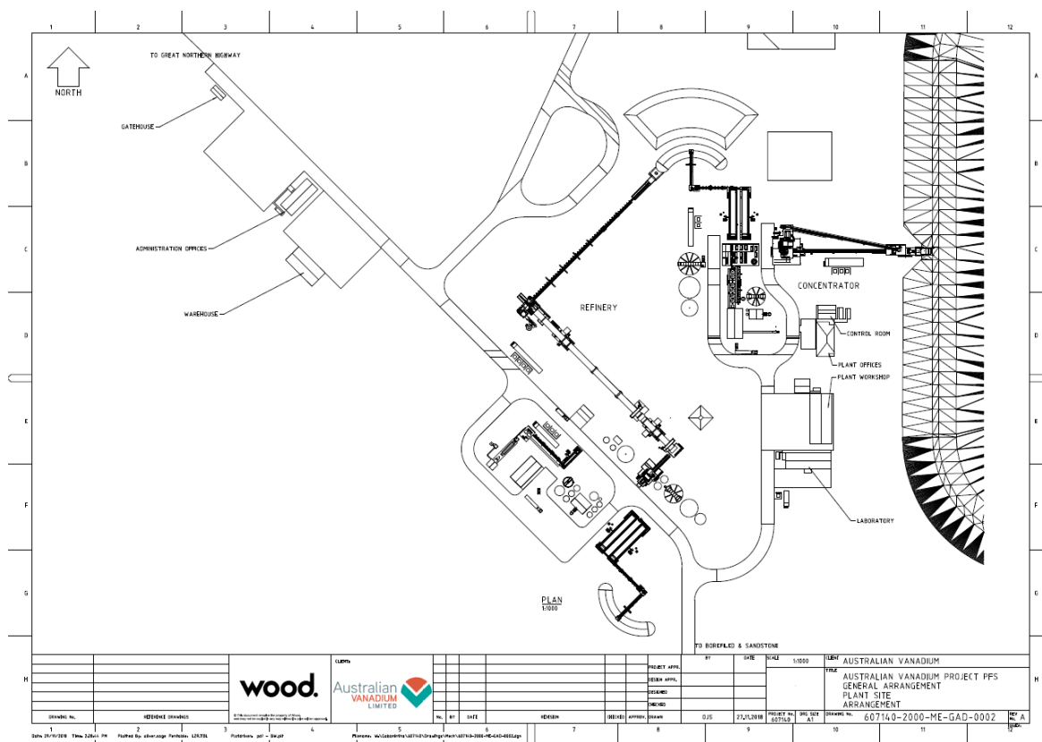
Figure 14 Process Plant Area General Arrangement Drawing
