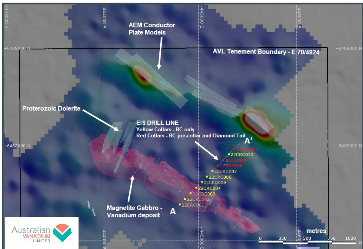
Figure 2: Plan view of EIS Drill Line with AEM imagery background and Plate Models
