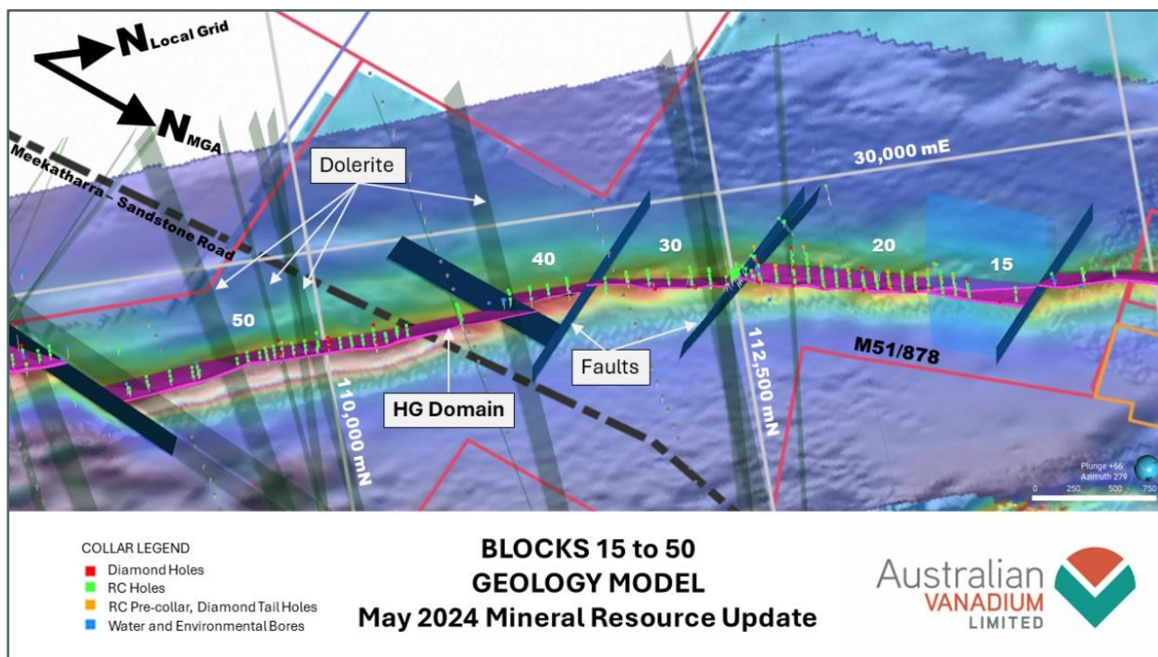
Figure 10 – Oblique View Looking Southwest – Block 15 to 50 geology model on regional magnetics composite image
