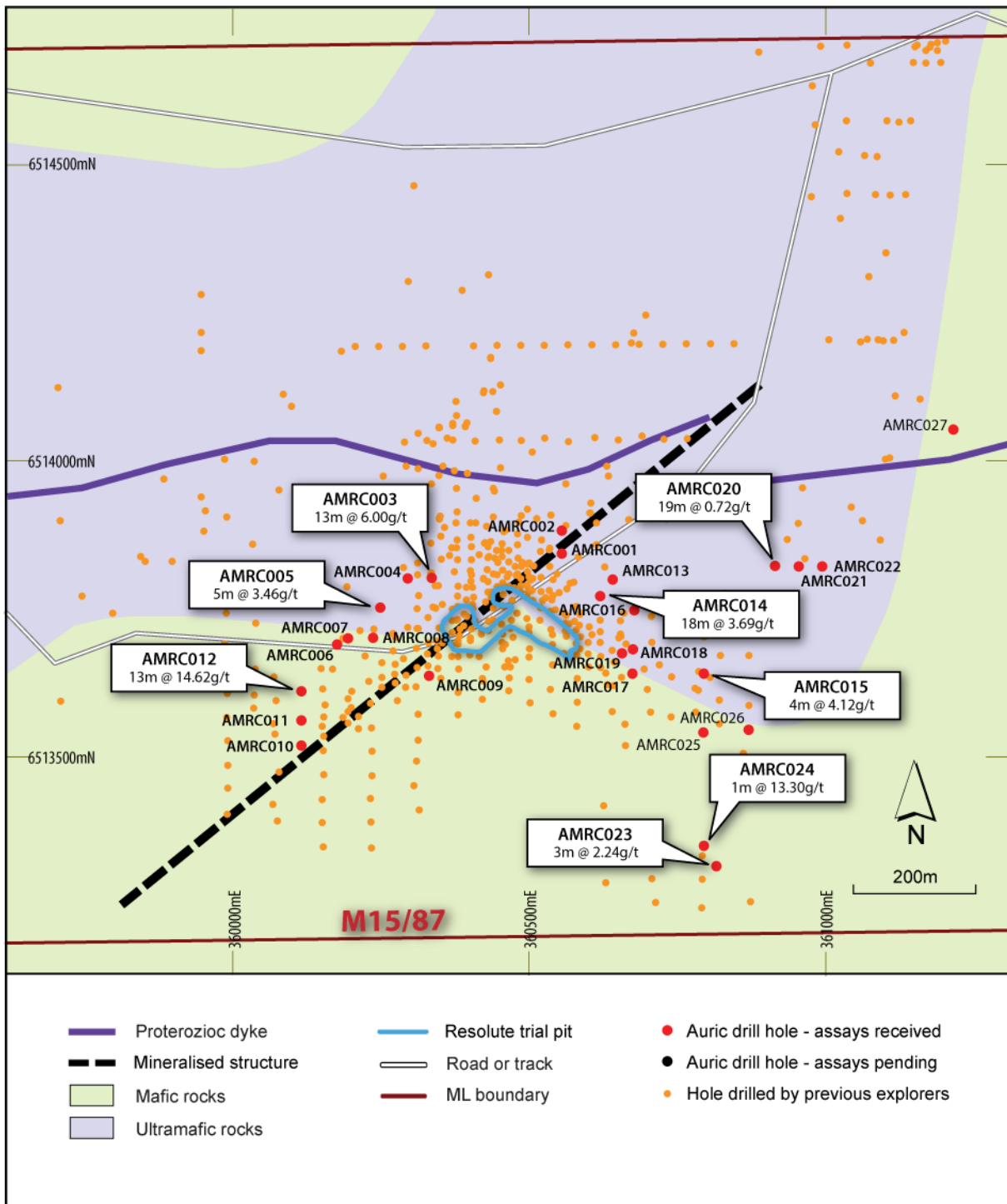
Figure 2. Munda drilling and geology
