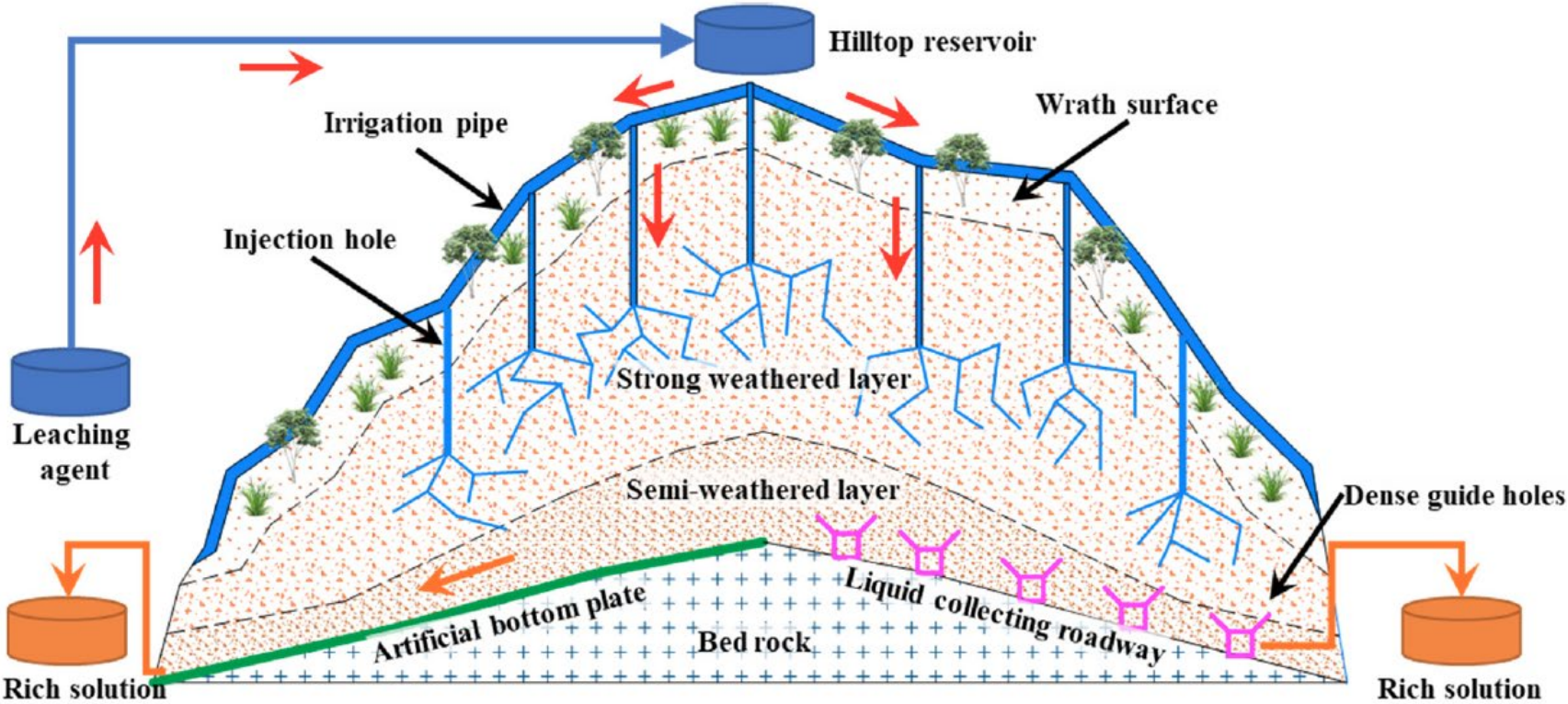
Schematic diagram of the in situ leaching process for rare earth ore
