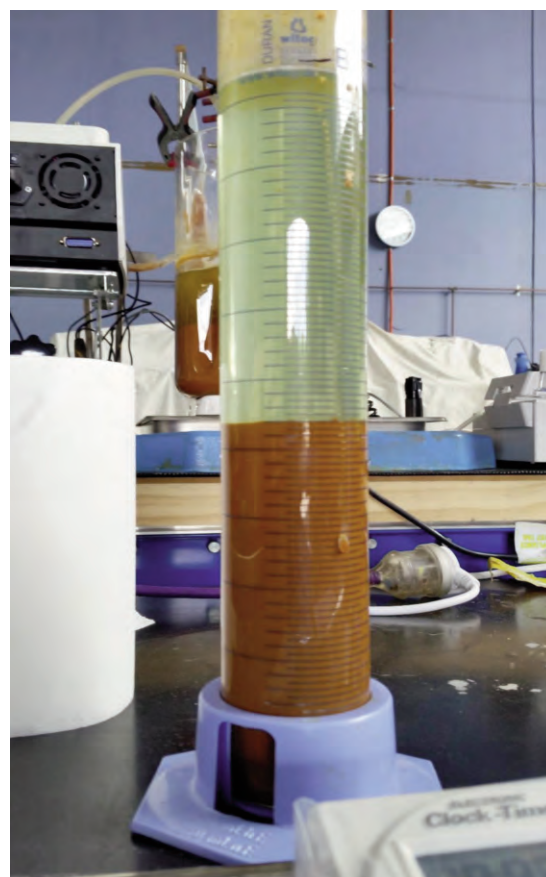
Figure 4: Results of solution neutralisation and Fe/Al removal batch test, showing excellent solid/liquid separation characteristics (Fe/Al brown precipitate in the lower portion, light green Ni/Co rich neutralised solution above)
