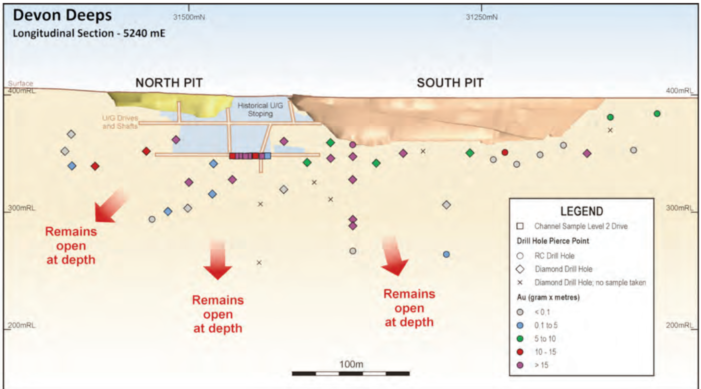
Figure 11. Long Section of the Devon Gold Mine
