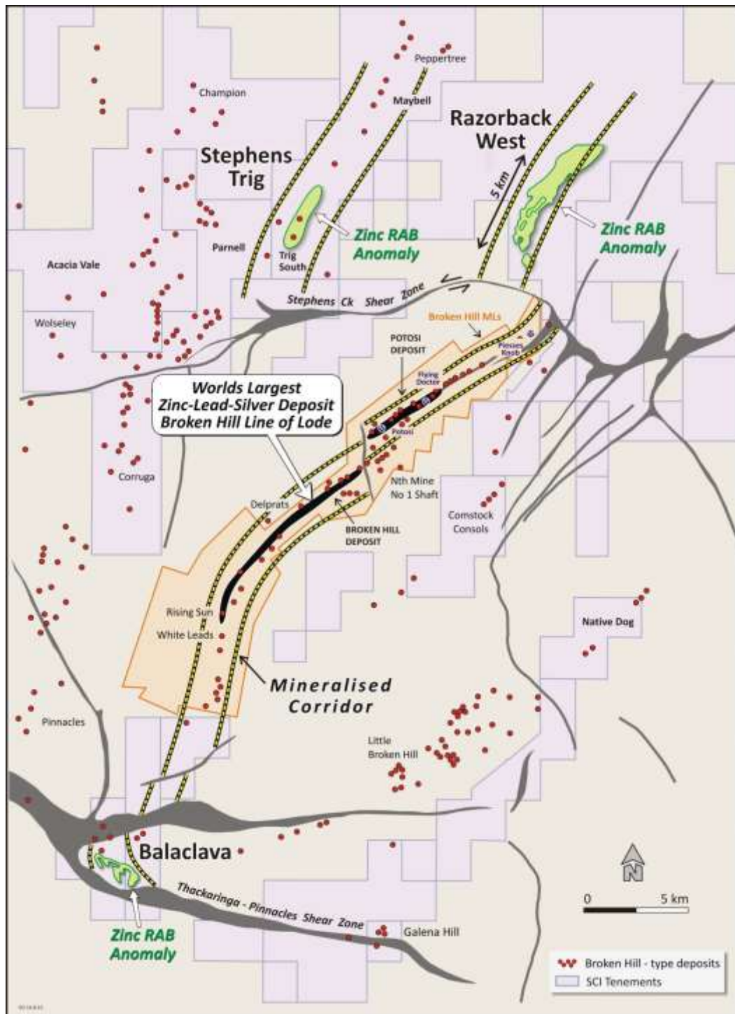
Figure 2. Broken Hill, showing the location and surface projection of the supergiant Broken Hill Deposit. It shows the relationship of the deposit to SCI tenements and specifically to the location of Razorback West to the north and Balaclava to the south. Interpretations suggest both Razorback West and Balaclava are fault-offset and/or fault-rotated extensions of the mineralised corridor which hosts Broken Hill.
