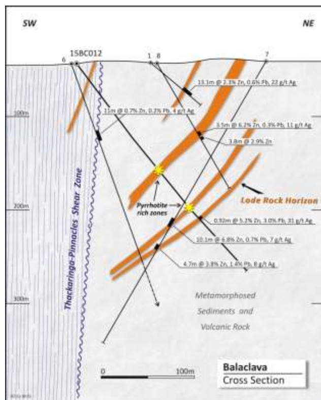
Figure 4. Cross-section at Balaclava showing hole 15BC012 in relation to historic holes. Holes have been projected into the plane of the cross-section (location shown in Figure 3).
