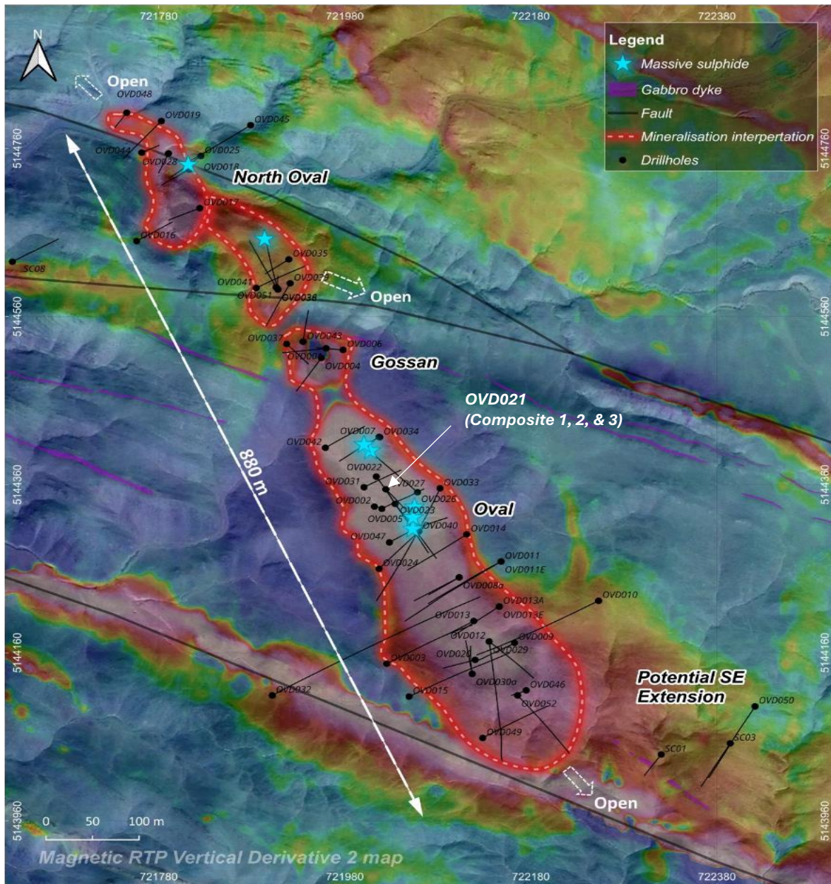
Figure 2. Location plan map of drillholes and metallurgical sampling location.
