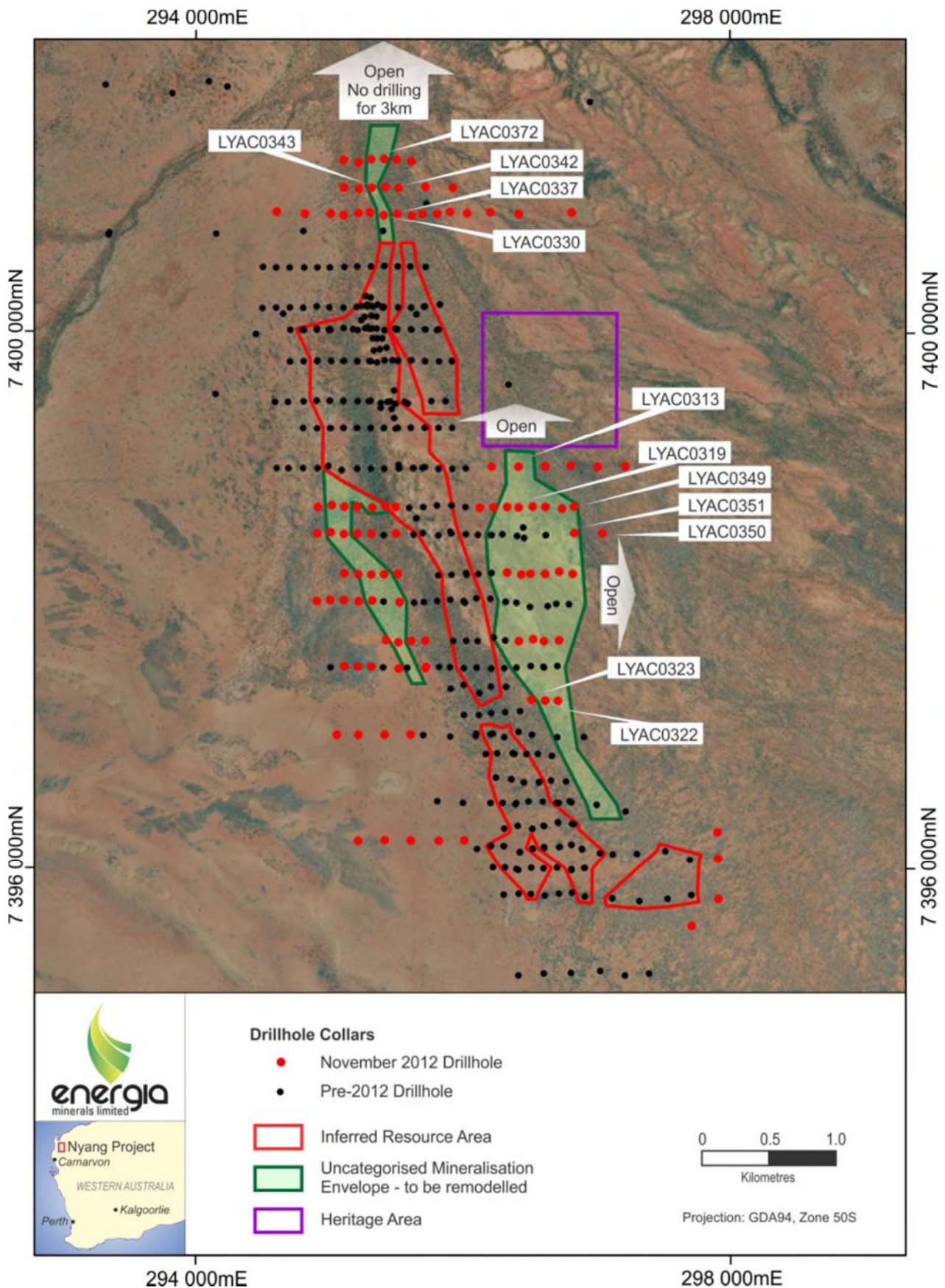
Figure 1 – Nyang Project showing location of Carley Bore Inferred Resource, Eastern Mineralised Zone, historic and November 2012 drilling.
