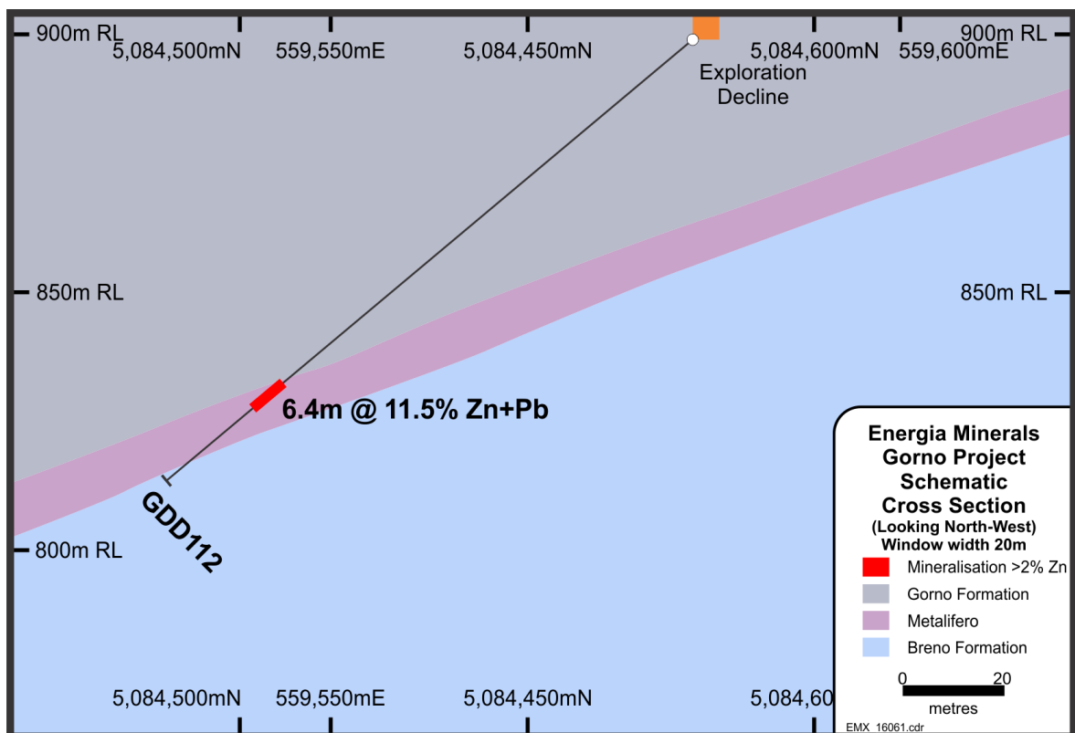
Figure 7: GDD112 Cross Section
