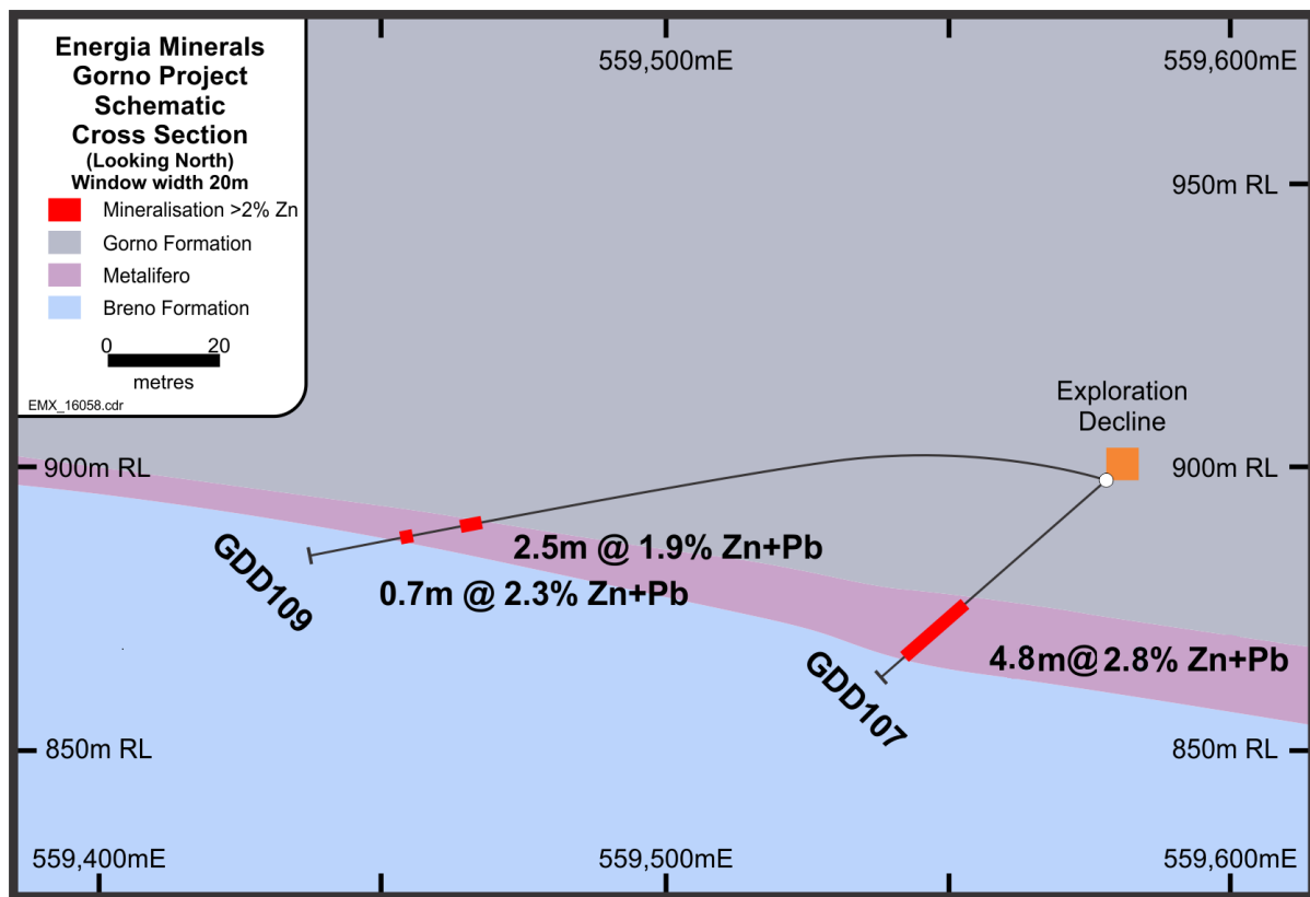
Figure 4: GDD109 Cross Section
