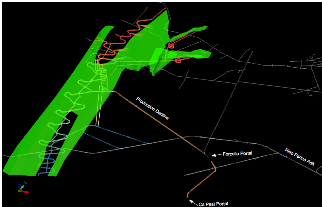
Figure 2: Colonna Zorzone Preliminary Mine Layout
