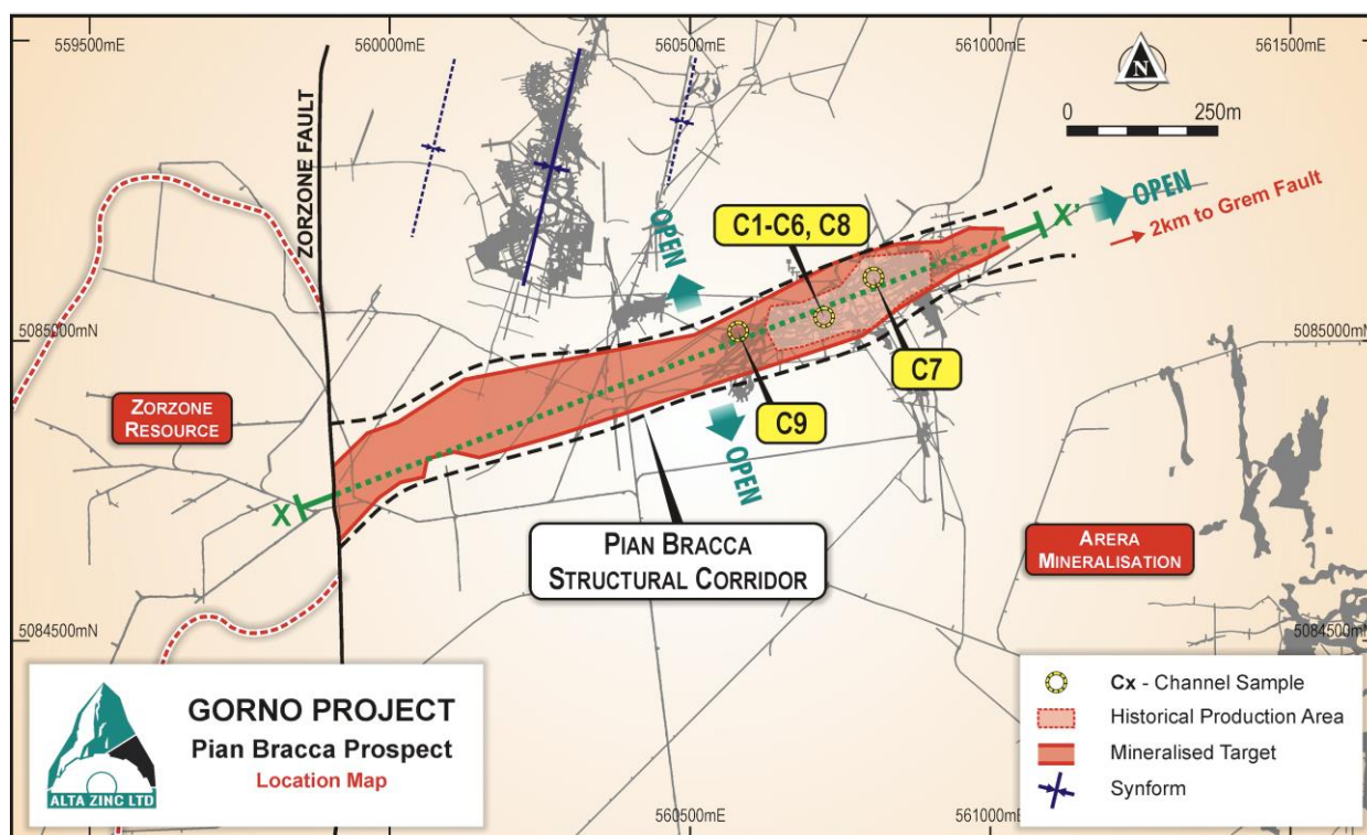
Figure 2: Plan view showing the location of the new channel samples (C8 & C9) within the Pian Bracca zone & the channel samples taken previously (C1-C7)
