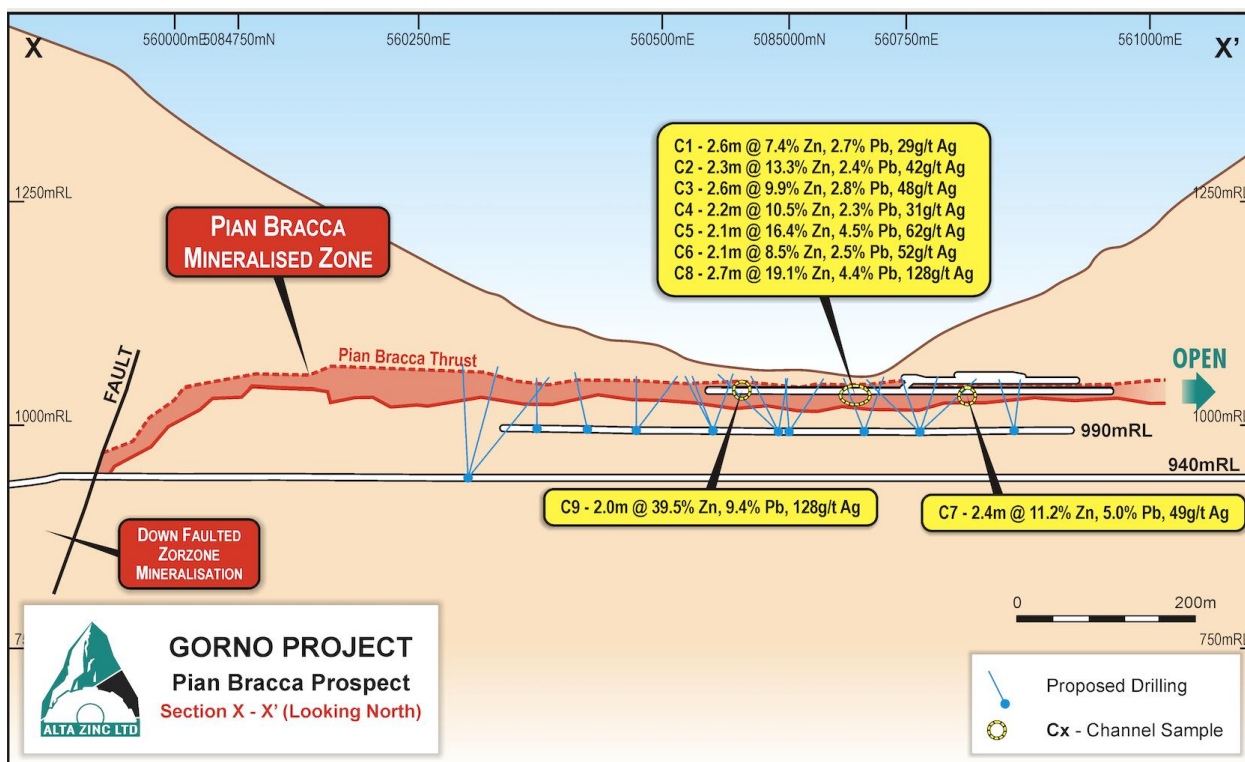
Figure 3: Long section through the Pian Bracca zone showing the new (C8 & C9) & previous (C1-C7) channel sample results & the proposed drilling of the zone from the existing access
