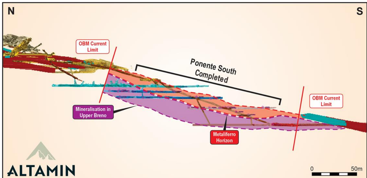
Figure 3: N-S sections through Ponente South showing current limits of block model
