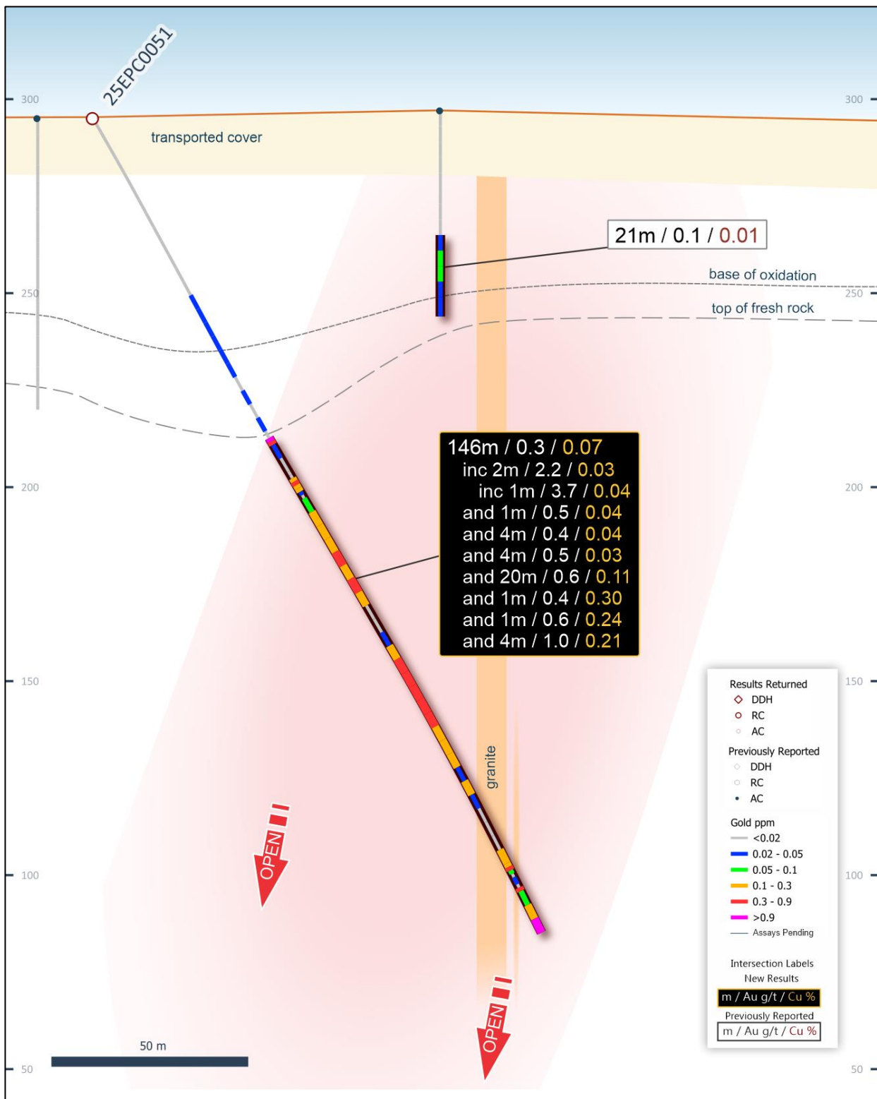
Figure 15: RPS (Poblano) deposit GDA SW-NE cross-section: Showing drill hole gold-copper drill intercepts including 25EPC0051. NB: Refer to Figure 11 for location information and 50m elevation (RL), looking toward 330° GDA2020 / MGA Zone 51 Grid.
