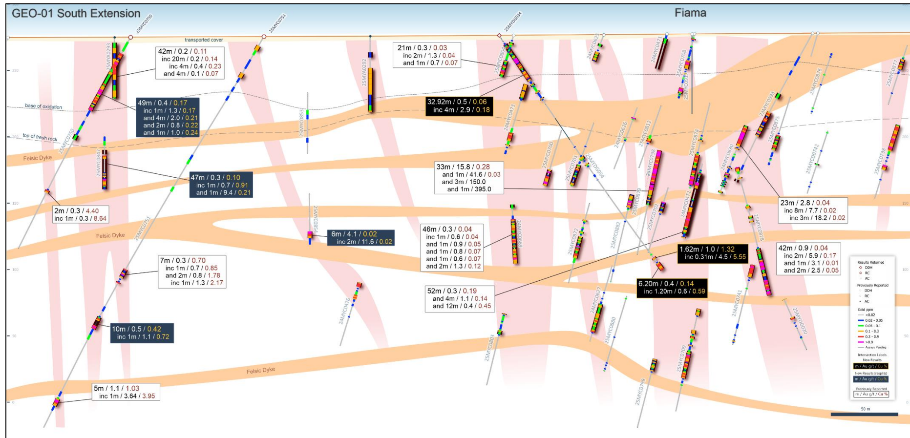
Figure 6: Fama and Rizzo deposit GDA NE-SW cross-section: Showing drill hole gold-copper drill intercepts including 25MYDG034 (Fama) and 25MYC0750 (Rizzo). Both the Fama and Rizzo deposits remain open down dip and along strike for multiple zones of mineralisation. NB: Refer to Figures 2 to 4 for location information and 50m elevation (RL) grid, cross-section plane of drill holes 25MYDG034 and 25MYC0750 looking toward 330° GDA2020 / MGA Zone 51 Grid.
