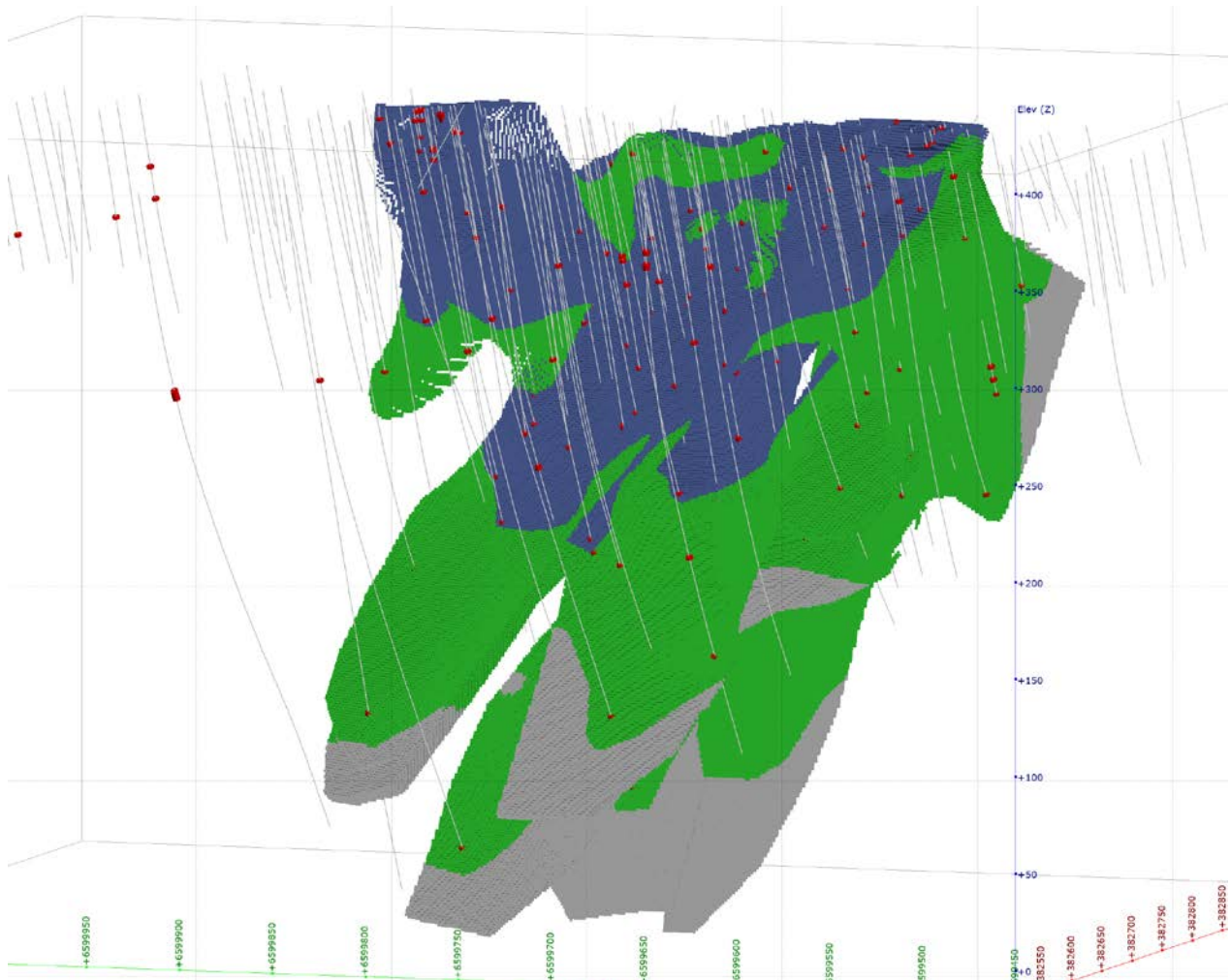
Figure 8: Oblique image looking NE showing Myhree Resource classification (blue=Indicated, green=Inferred, grey=Unclassified).
