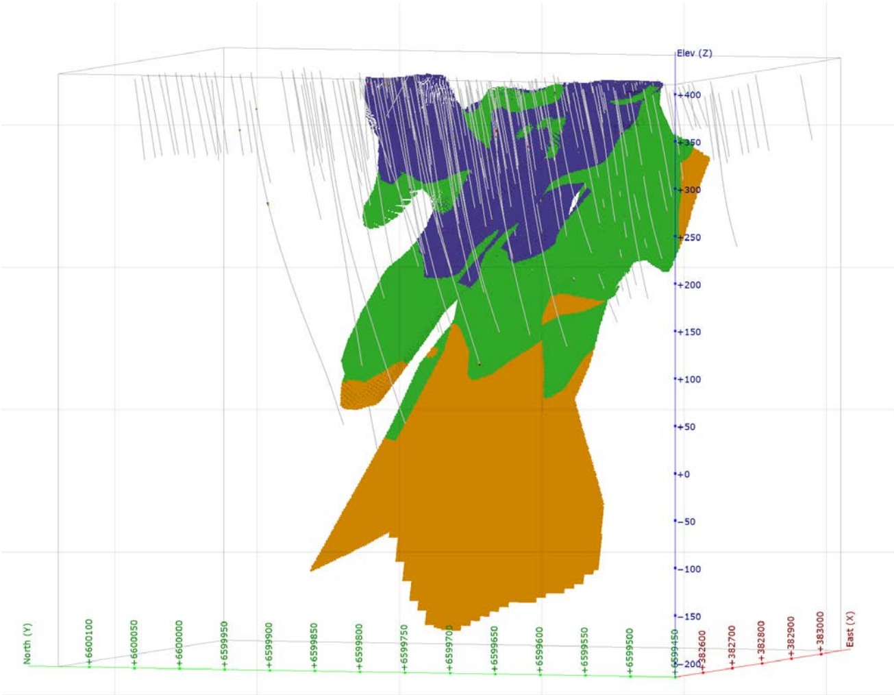
Figure 9: Oblique image looking NE showing Myhree Resource (blue=Indicated, green=Inferred) and Exploration Target (orange).
