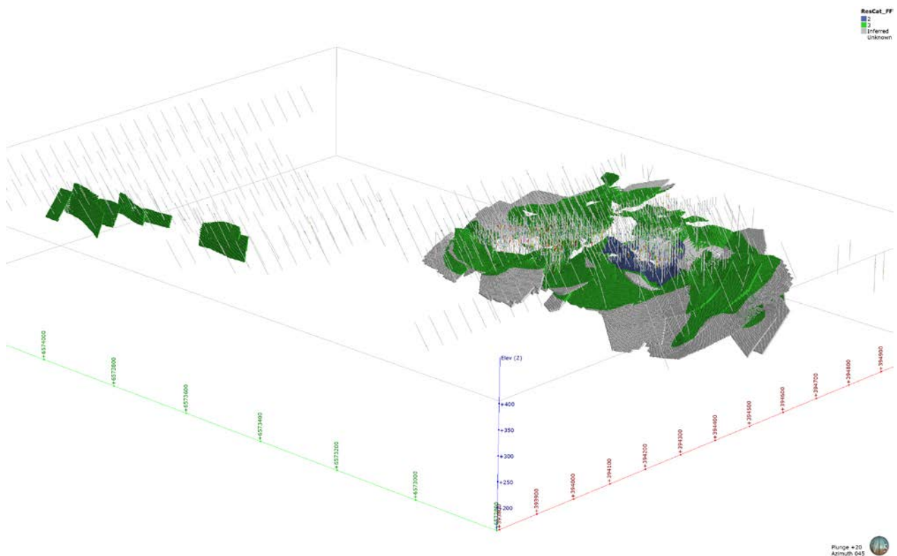
Figure 7: Oblique image looking NE showing Resource classification (blue=Indicated, green=Inferred, grey=Unclassified) for Fingals Fortune.
