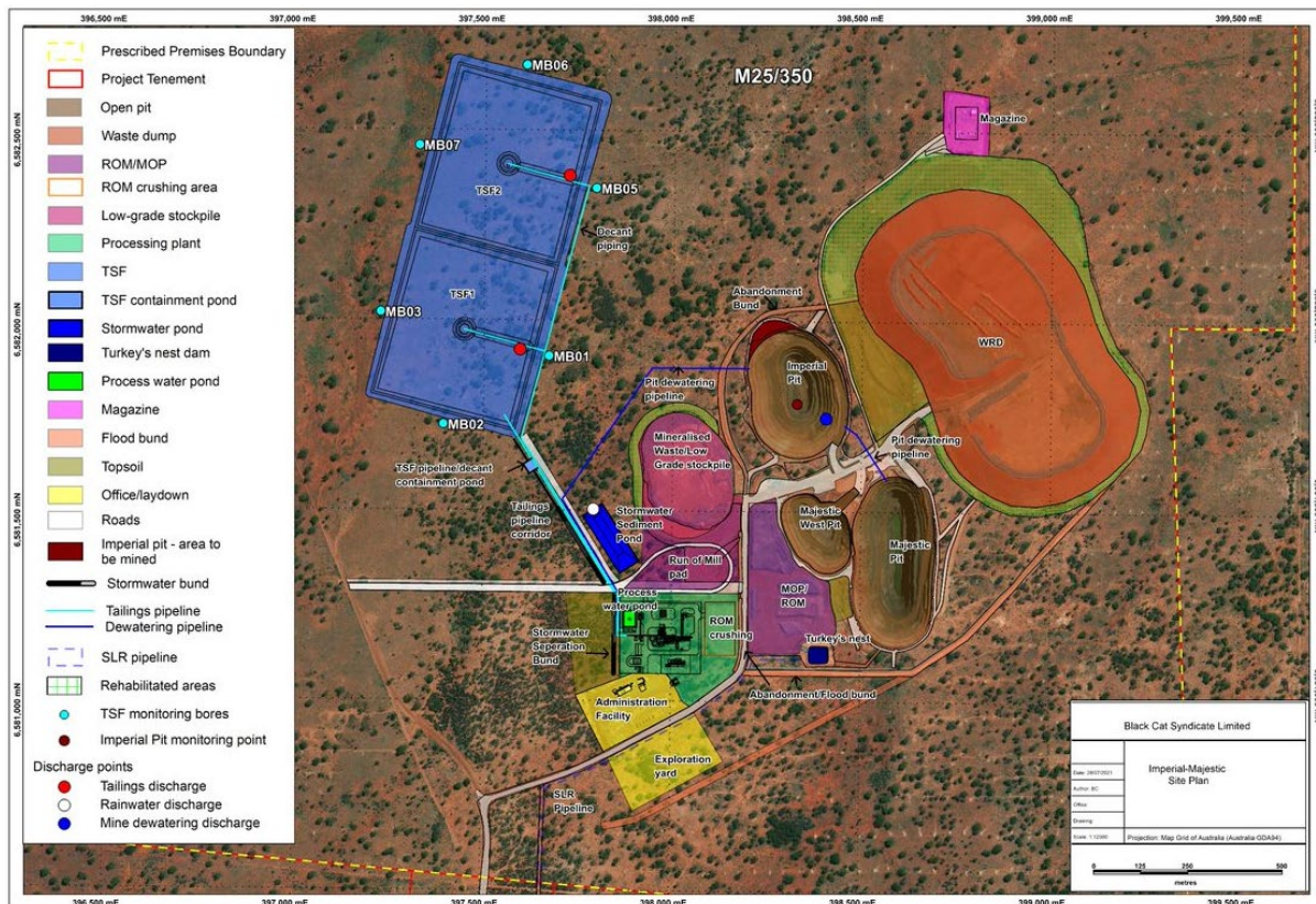
Figure 4: Site plan of Black Cat's approved gold processing facility and associated infrastructure at Majestic
