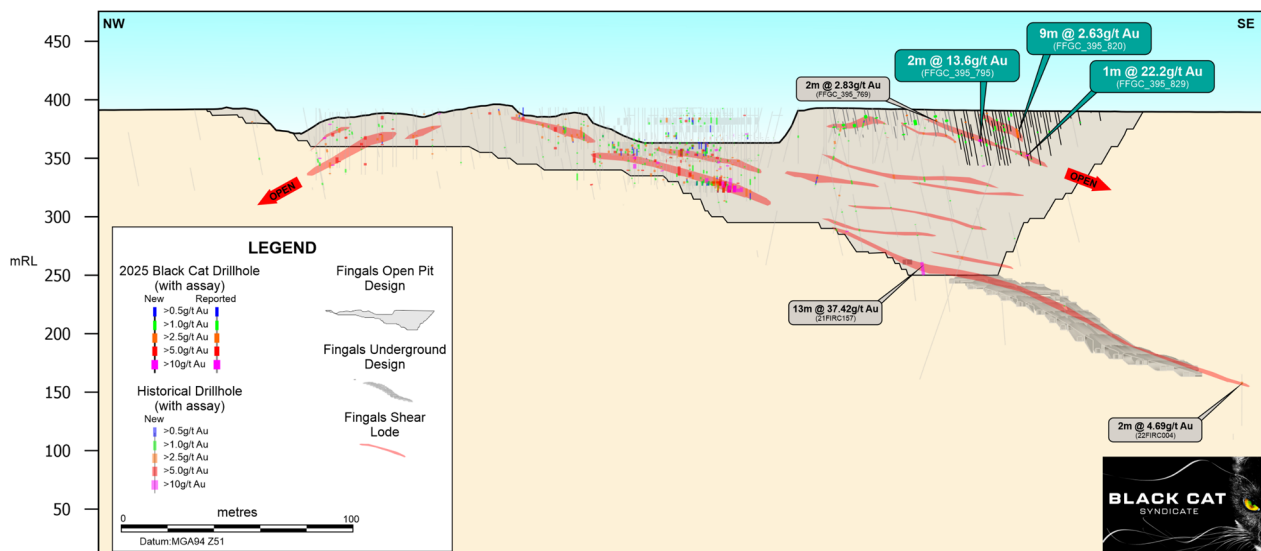
Figure 4: Longsection (see Figure 3) through Fingals showing the planned open pit and initial underground design along with new drilling defining unmodelled high-grade gold zones in the upper southern part of the pit.
