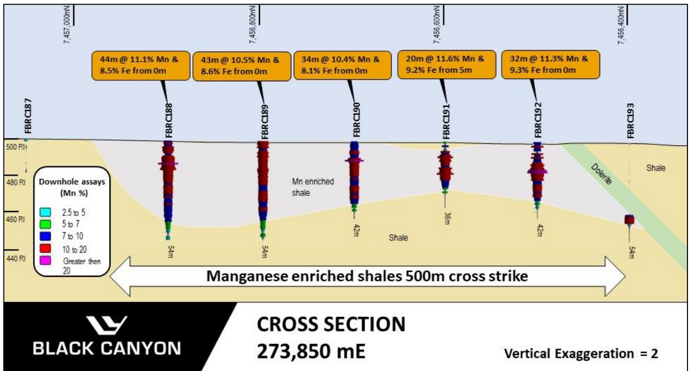
Figure 2. LR1 deposit cross section 273,850mE showing significant results from the LR1 drill program (looking east)
