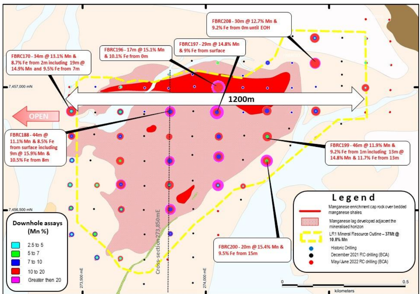
Figure 1. LR1 deposit drill plan showing significant drill results and downhole drill results projected to surface over mapped geology (BCA earning 75%)
