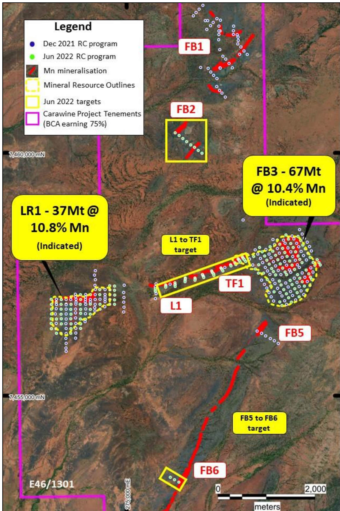
Figure 3. Flanagan Bore Project - FB3 & LR1 Mineral Resource outlines and additional drill targets at FB1, L1, TF1 and FB6 (Black Canyon (51%) earning up to 75%)
