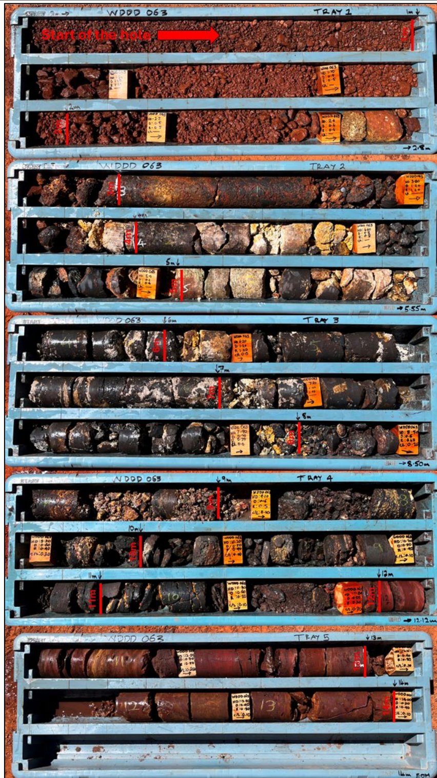
Figure 2. Drill hole WDDD063 twinning hole WDRC063 that intersected 10m @ 27.7% Mn & 7.6% Fe from 4m including 3m @ 39.6%Mn & 3.9% Fe from 10m. Assays quoted from the equivalent interval from WDRC063 to the twin diamond hole will vary due to geological variation and recovered core. Manganese mineralisation can be observed from 3 to 12m increasing grade with depth. Downhole metre marks are drawn on the core and tray ribs.
