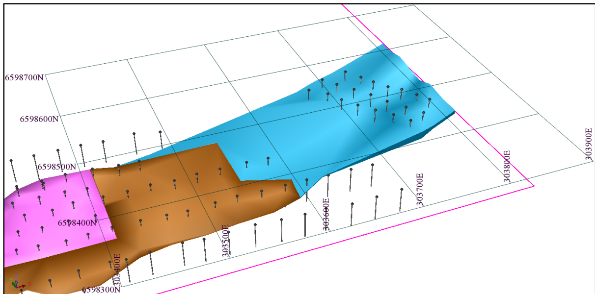
Figure 2: NE extensional drilling at the Lost Dog prospect showing the trend of mineralisation is open to the NE
