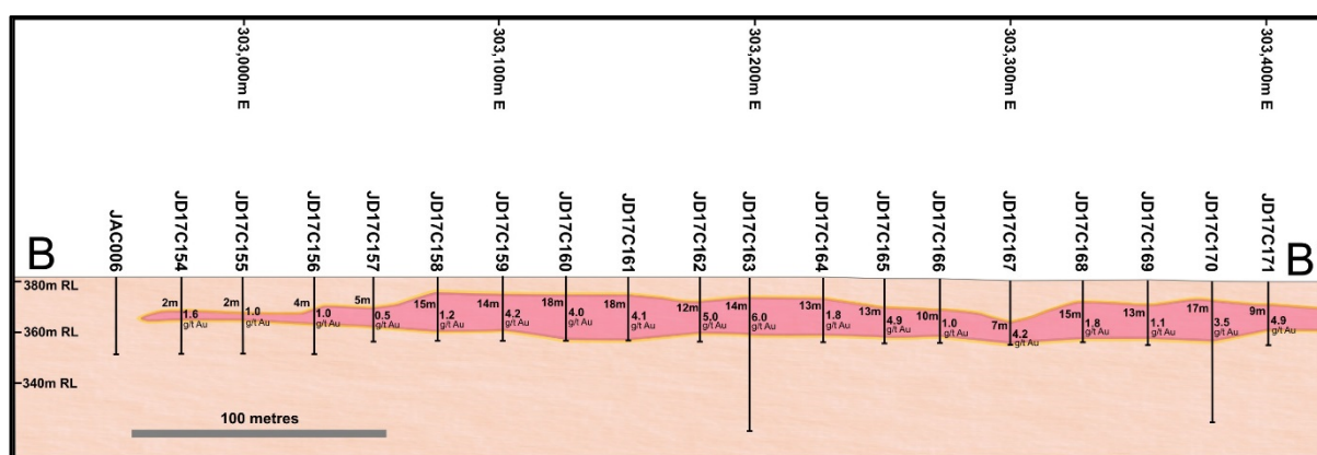
Figure 7: Long section B – B' of the East Arm of the Jaurdi palaeochannel
