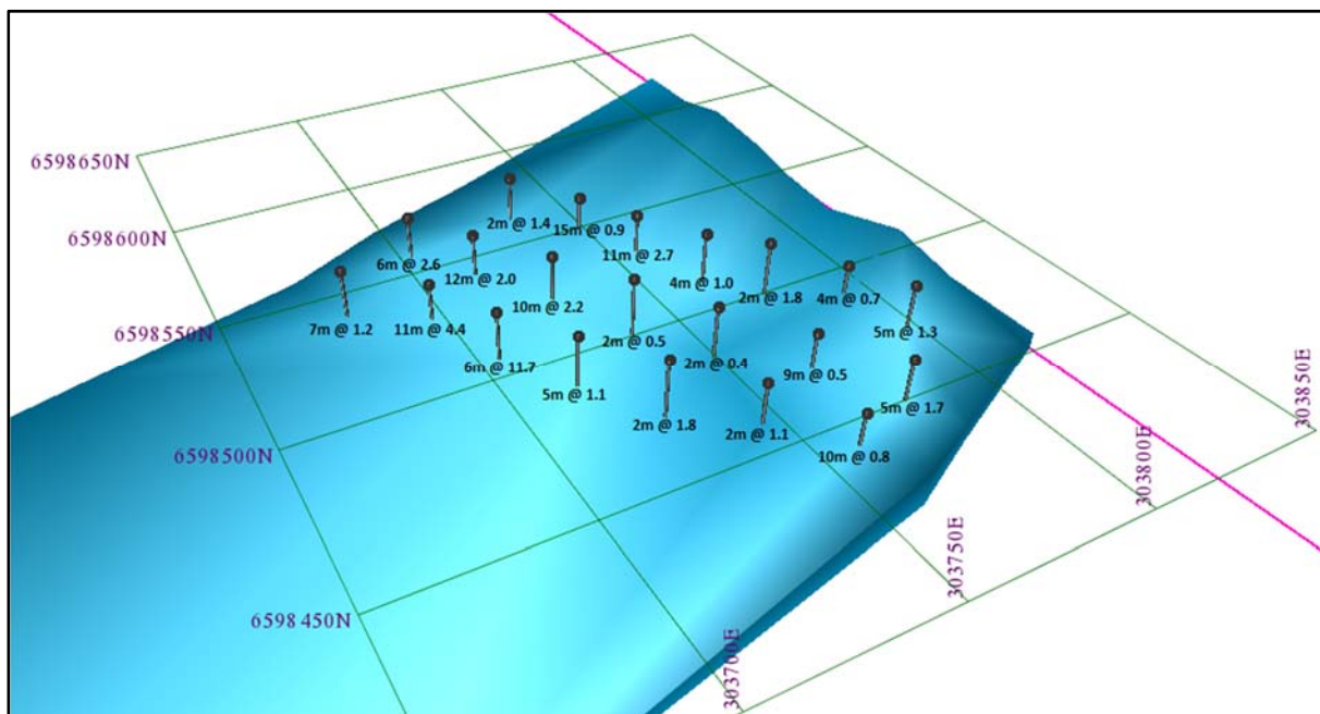
Figure 3: Drill results from the NE extension drilling showing mineralisation open in all directions
