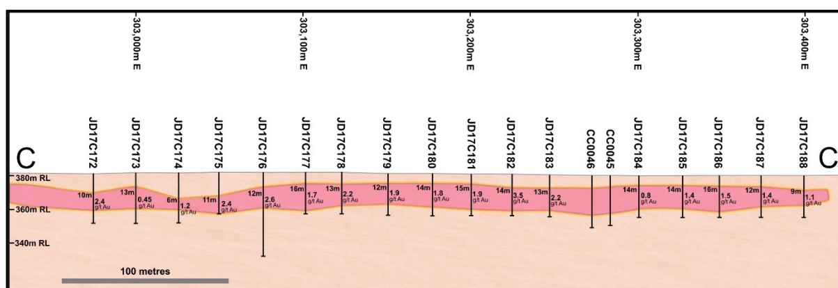
Figure 8 Long section C – C' of the East Arm of the Jaurdi palaeochannel
