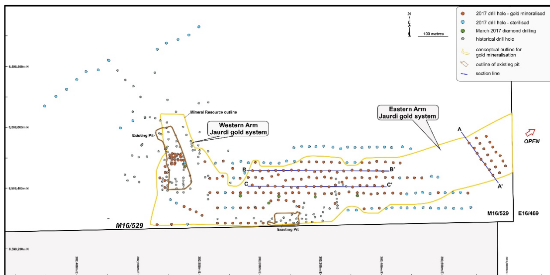
Figure 5: Plan of the Jaurdi palaeochannel showing the drilling which has defined both the Eastern and Western Arms
