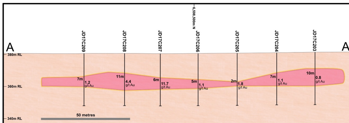
Figure 6: Cross section A – A' of the East Arm of the Jaurdi palaeochannel
