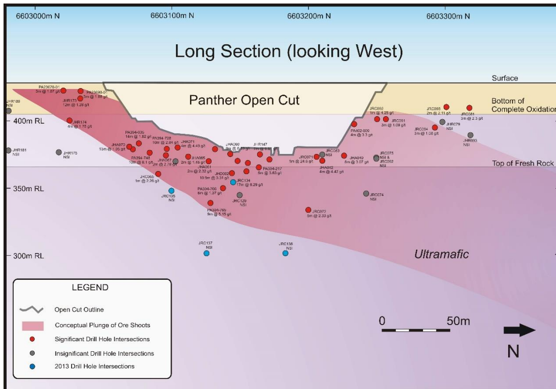
Figure 2: Long section showing the Panther mineralisation
