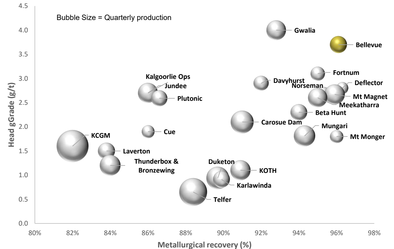
Recovered gold per tonne processed - Grade & Recovery 2
