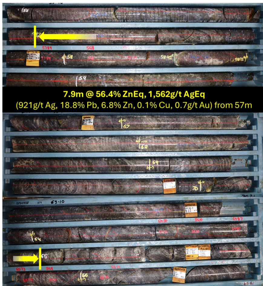
Figure 5 – Diamond drill core from BPD0038 within the Junction area of the Pinnacles Mine
