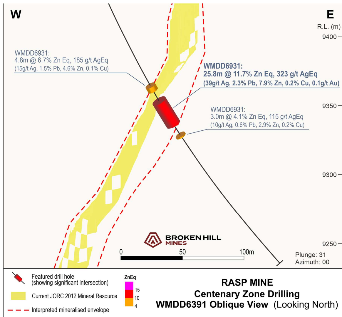
Figure 3 – Oblique view of WMDD6391 showing significant increase on modelled thickness and grade
