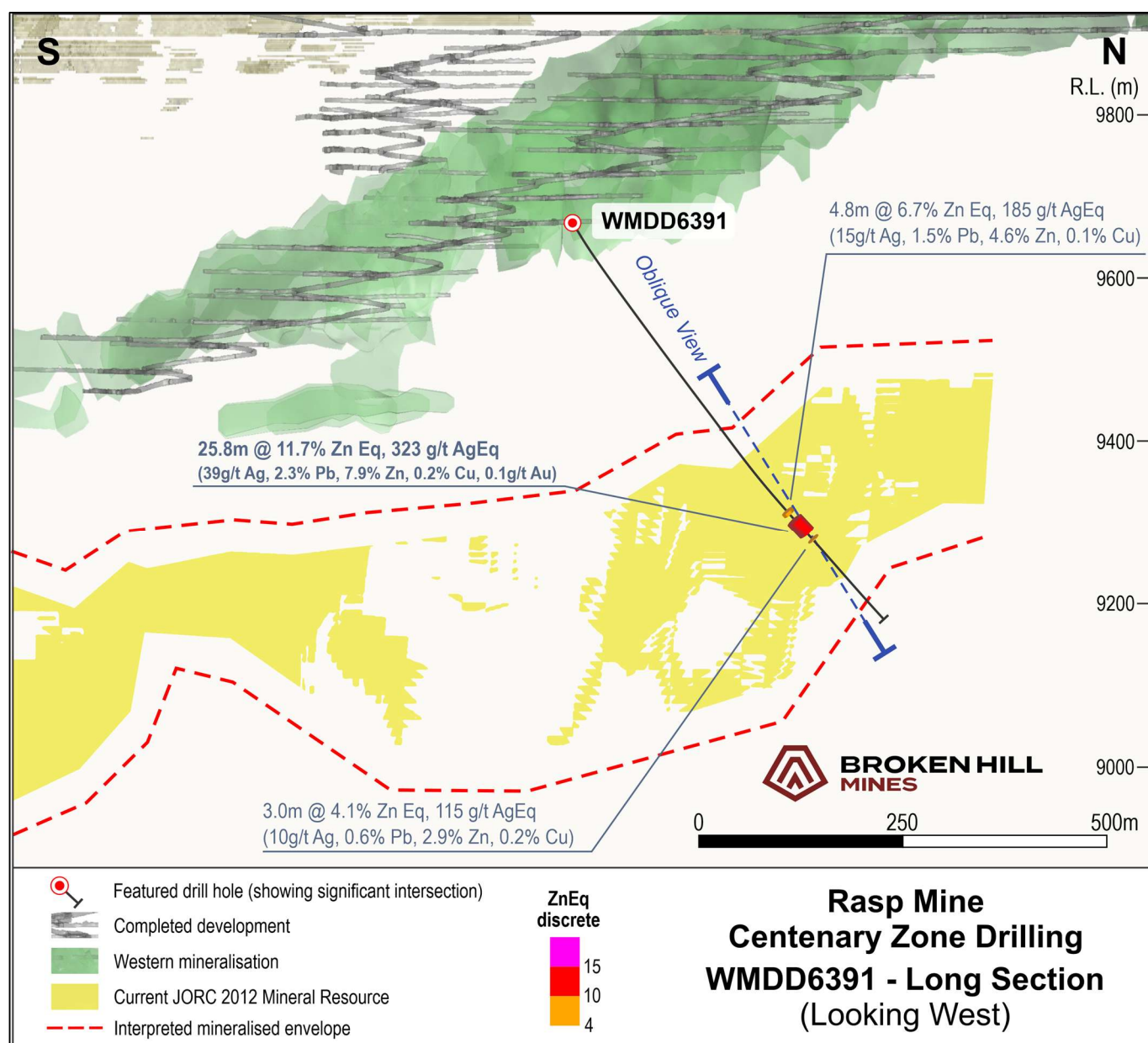
Figure 2 – Long section of the Centenary Zone within the Broken Hill ore body
