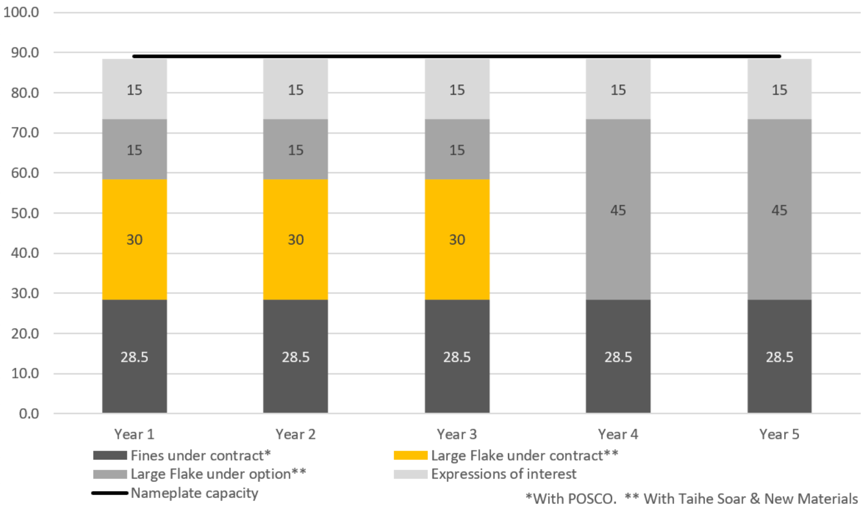
Mahenge Offtake for Module 1 (89ktpa)
