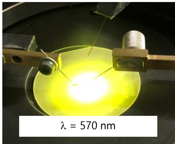
RPCVD p-GaN grown at low temperature
