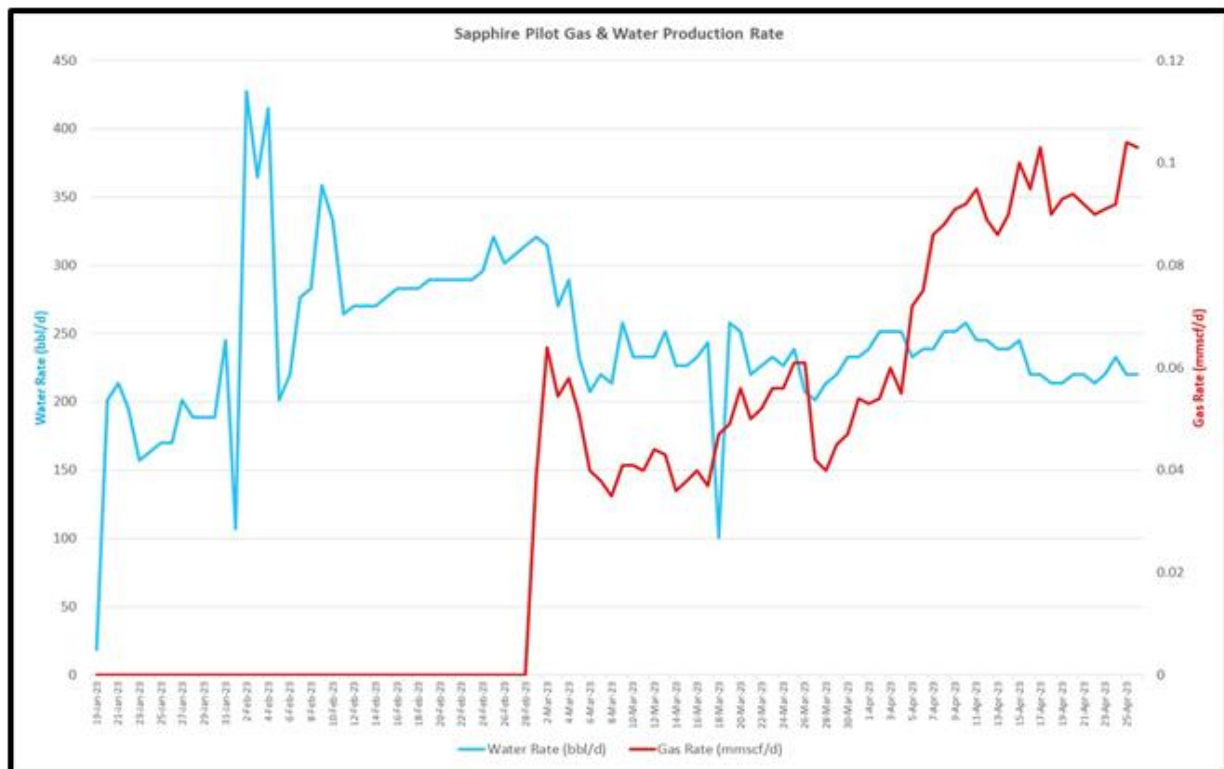
Figure 1: Graph showing gas rate increasing with time as water rate stabilises.
