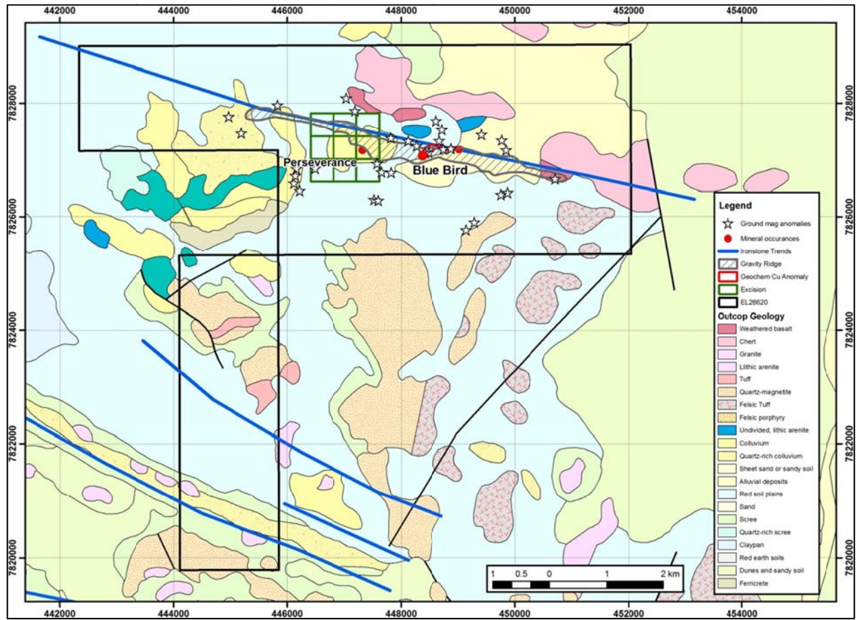
Figure 5 – Regional prospectivity map of the Barkly Cu-Au project. Blue lines show ironstone structural trends throughout the licence. Ironstones are prospective for other high-grade Tennant Creek style deposits.
