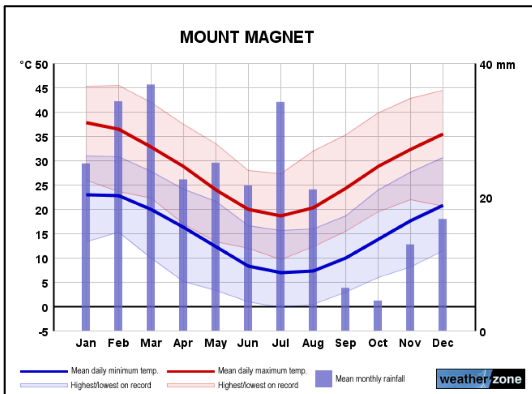
Figure 3: Mount Magnet climate
