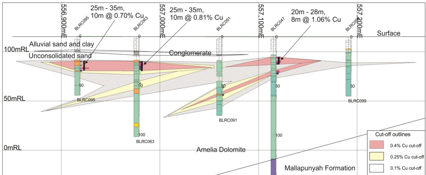
Figure 3: Section through oxide copper mineralisation, Lorella prospect
