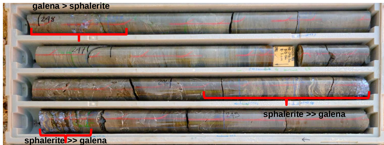
Figure 5 -Photograph of SHSD_185 drill core interval 244.6m to 248.04m showing massive sphalerite + galena replacement mineralisation intervals hosted in bedded carbonates of the Burt Range Basin.
