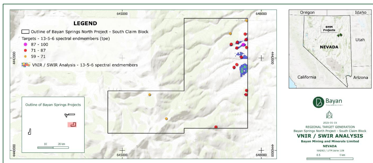
Figure 4: Bayan Springs North – Southern claim block - targets defined based on pyrite, stibnite and illite spectral endmembers
