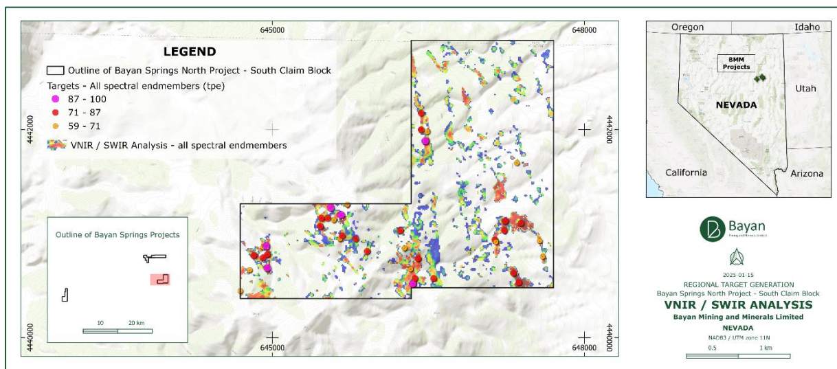
Figure 6: Bayan Springs North – Southern targets defined based on all spectral endmember
