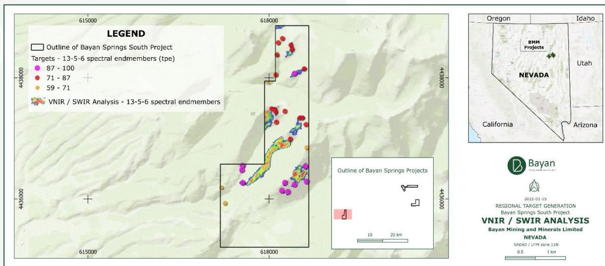
Figure 7: Bayan Springs South – targets defined based pyrite, stibnite and illite spectral endmembers
