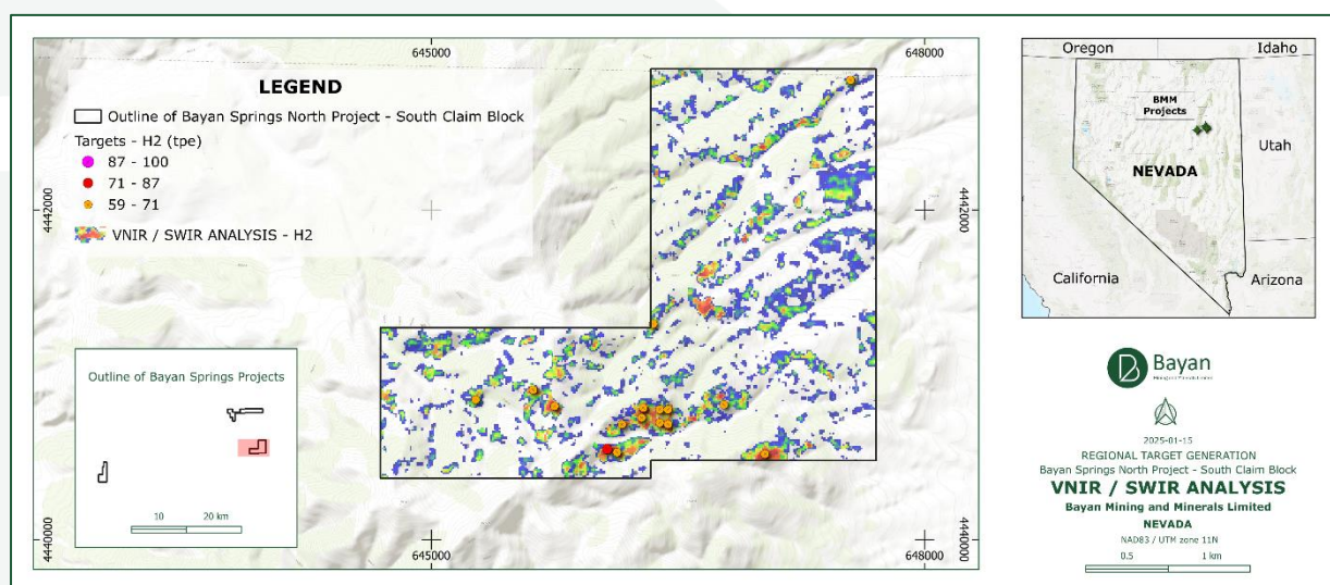
Figure 5: Bayan Springs North – Southern targets defined based on H 2 spectral endmember
