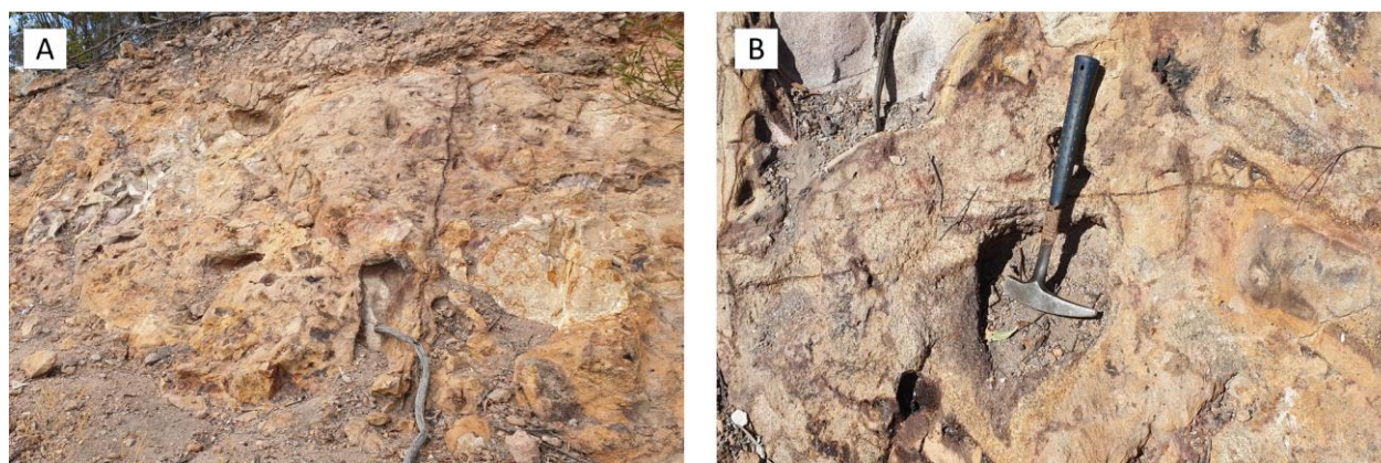
Figure 2. Examples of the strongly altered Seventy Mile Mount milled breccia and exhibiting clasts of granodiorite, volcanics, fine grained intrusives and chert.
