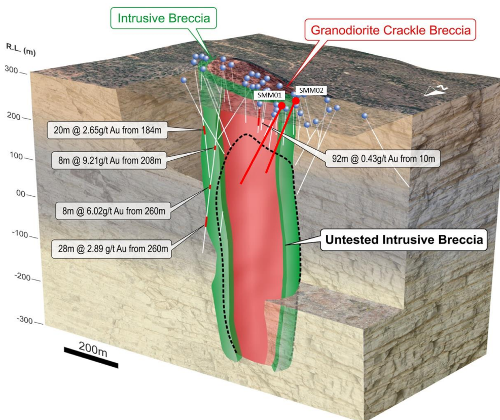
Figure 3. 3D geological model of the Seventy Mile Mount prospect, looking south, showing mapped geology (i.e. granodiorite crackle breccia (red) and altered polymictic milled breccia (green) and historic drill holes with gold assays, and proposed drill holes SMM01 – SMM02 (red).
