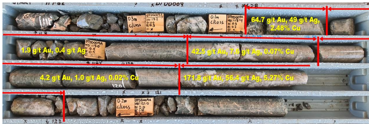
Figure 4 - DTDD009 HQ Drill Core Intersection of 2.25m @ 54.9 g/t Au, 20.6 g/t Ag &amp; 1.52% Cu from 118.4m. This intersection is typical of the mineralisation observed in the historic Dittmer Mine.
