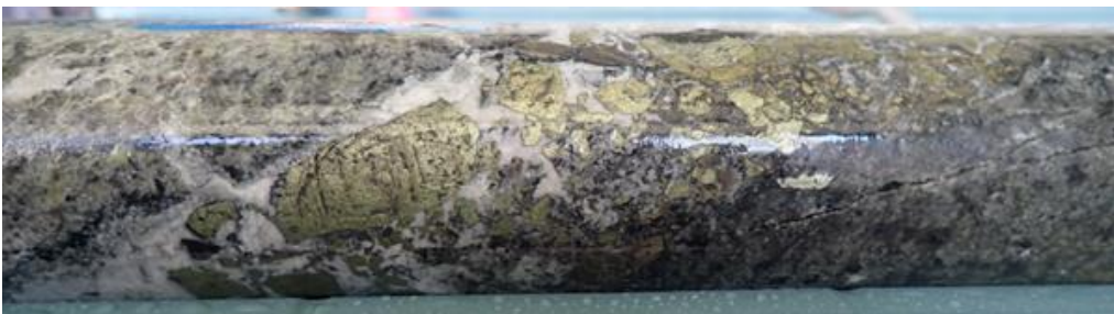
Silica-sericite altered, sheared granodiorite crosscut by quartz-carbonate-chalcopyrite veins (BRUDD003: 118.3 – 118.5m)
