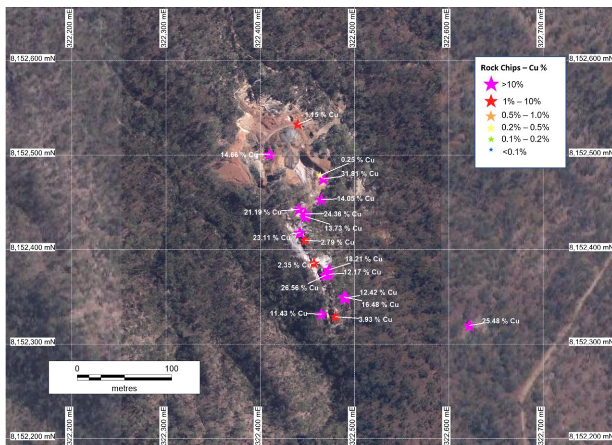
Figure 4 – Mount Molloy mine area showing rock chip sample locations with copper assay results.
