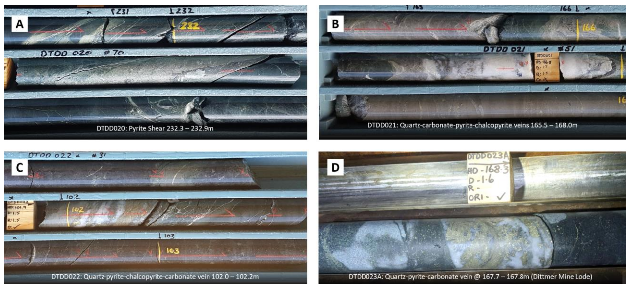
Figure 5 – Examples of mineralisation encountered in recent Dittmer drilling (A) Pyritic shear zone in DTDD020 (232.3 – 232.9m); (B) Quartz-carbonate-pyrite-chalcopyrite veins in DTDD021 (165.5 – 168.0m); (C) Quartz-pyrite-chalcopyrite-carbonate vein in DTDD022 (102.0 – 102.2m); (D) Down-dip extension of mine lode in DTDD023A (167.7 – 167.8m).
