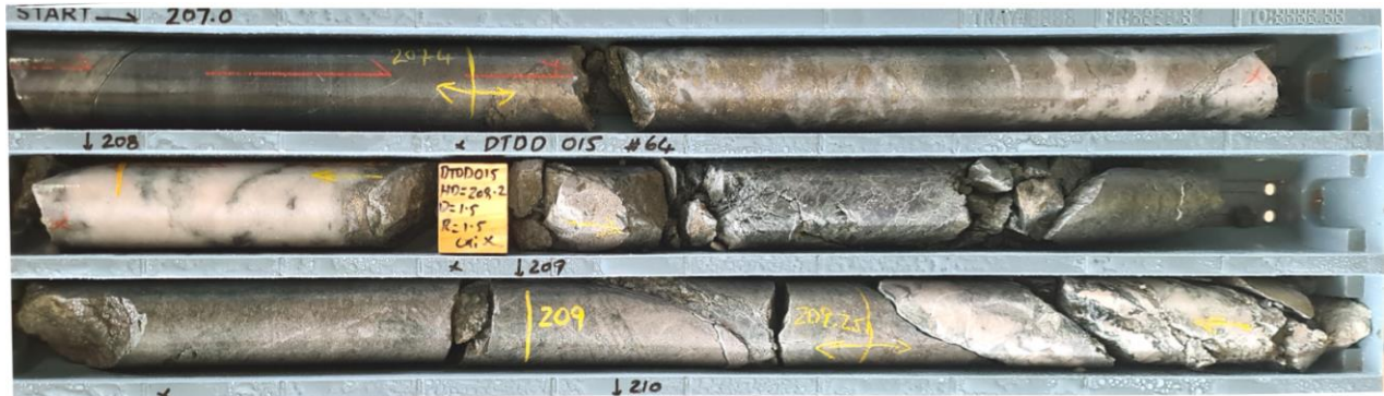
Figure 2 – Dittmer drill hole DTDD015 core tray containing sheared volcanics overprinted by quartz-pyrite-chalcopyrite veins (207.4 – 209.65m) with reported assay results of 2.25m @ 8.68 g/t Au, 2.8 g/t Ag & 0.25% Cu (207.4 – 209.65m), including 0.4m @ 37.62 g/t Au, 9.3 g/t Ag & 1.38% Cu (209.25 – 209.65m).
