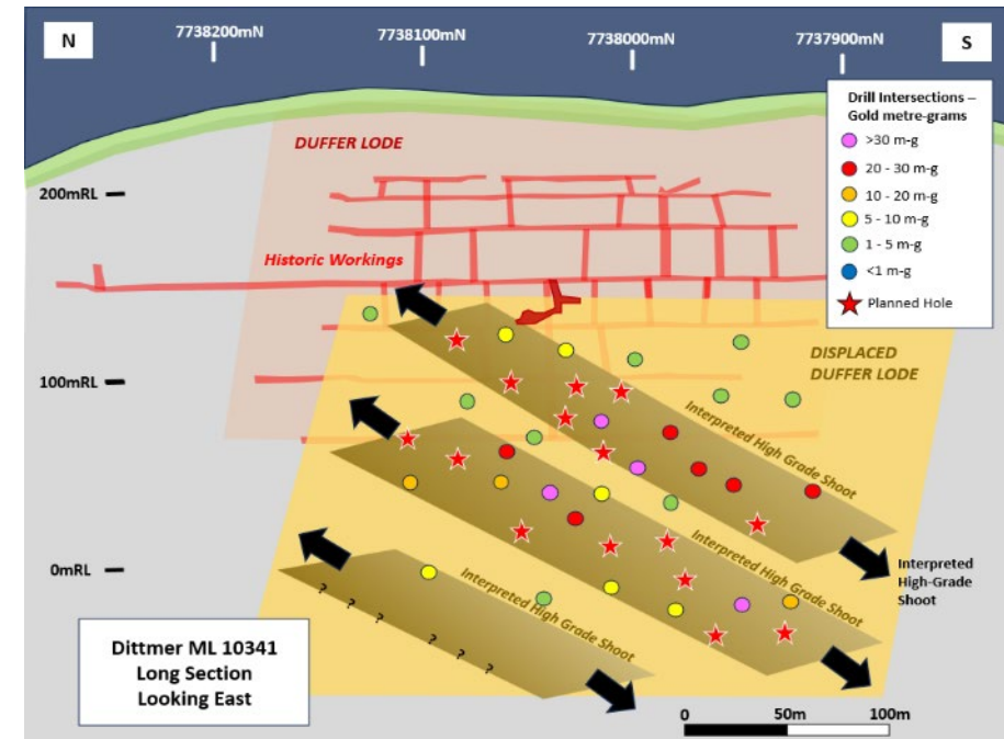
Infill Drill Design at Dittmer from Underground
