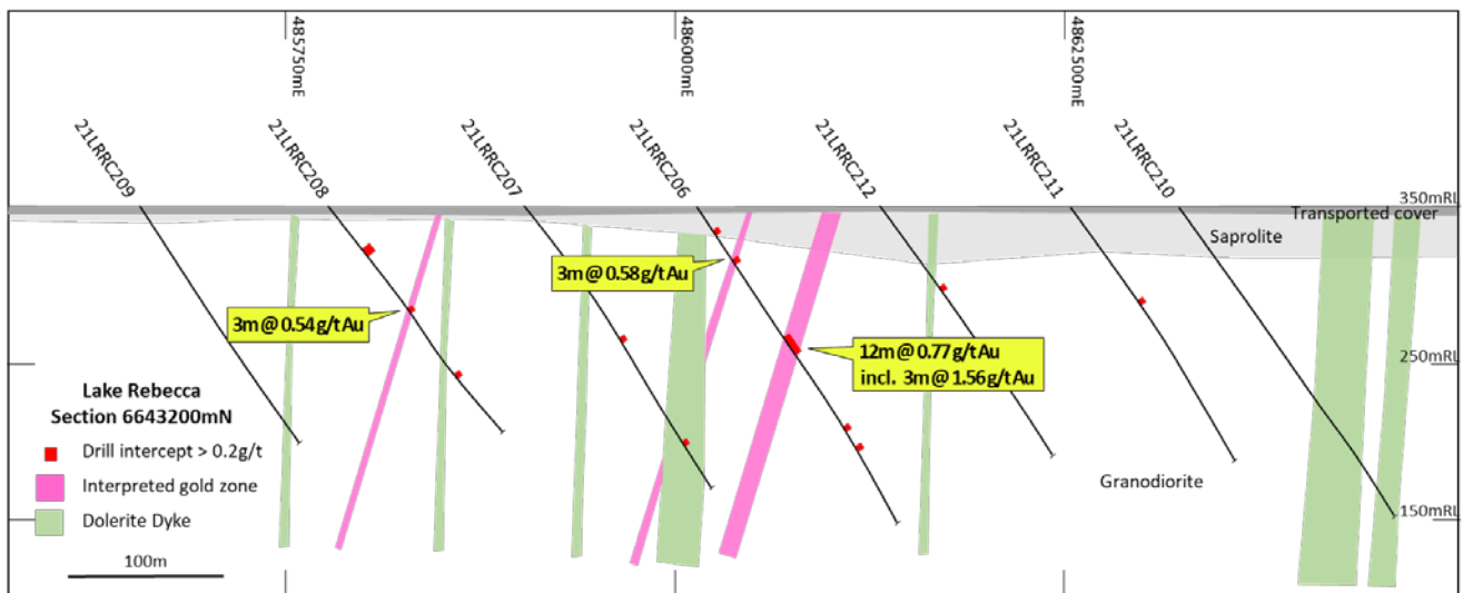
Figure 2: Cross Section 643200mN showing interpreted geology and mineralised intercepts above 0.5g/t Au annotated
