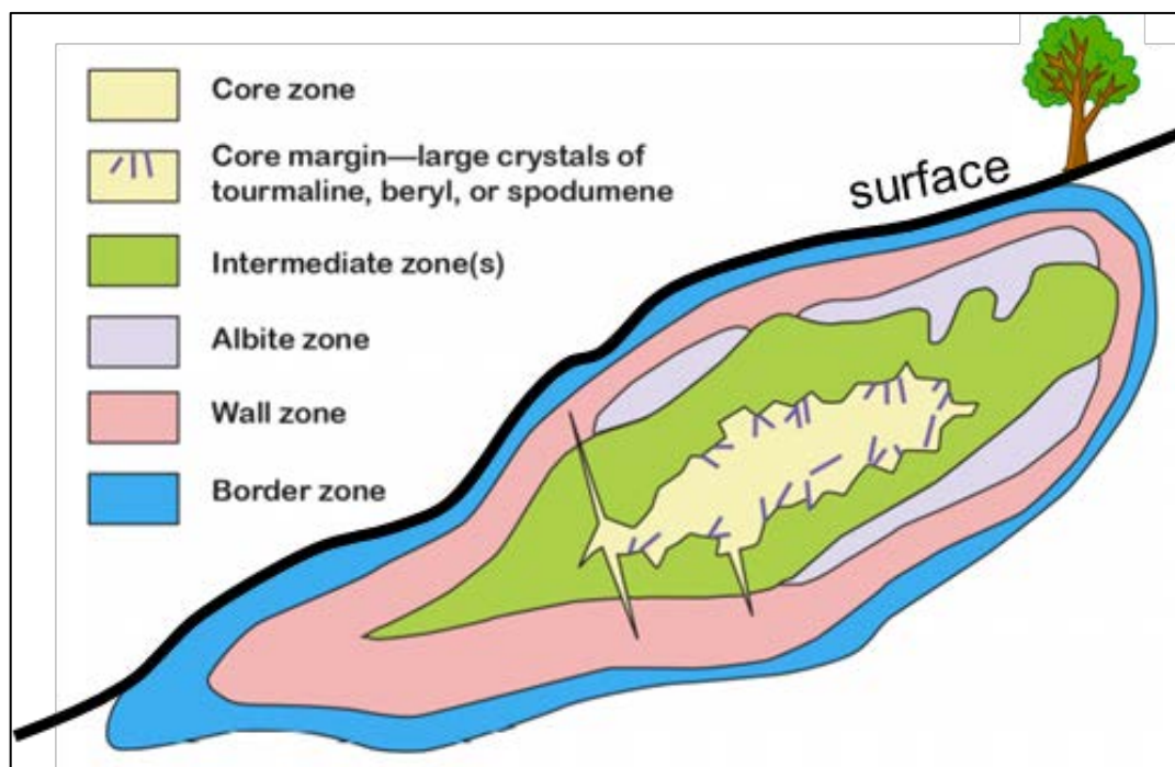
Figure 3: Deposit scale zoning (the result of fractionation as minerals precipitate out of the molten magma) in an idealised pegmatite (modified, Bradley and McCauley, https://pubs.usgs.gov/of/2013/1008/OF13-1008.pdf )
