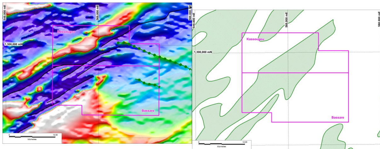
Figure 2: Tenkodogo Project regional aeromagnetic image (left) and simplified greenstone geology (right).
