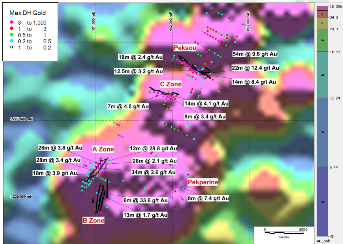
Figure 1: Southern Intiedougou Permit surface expression of gold mineralisation with RC and diamond drilling intercepts and prospects (labelled) over gold in soil geochemistry image.
