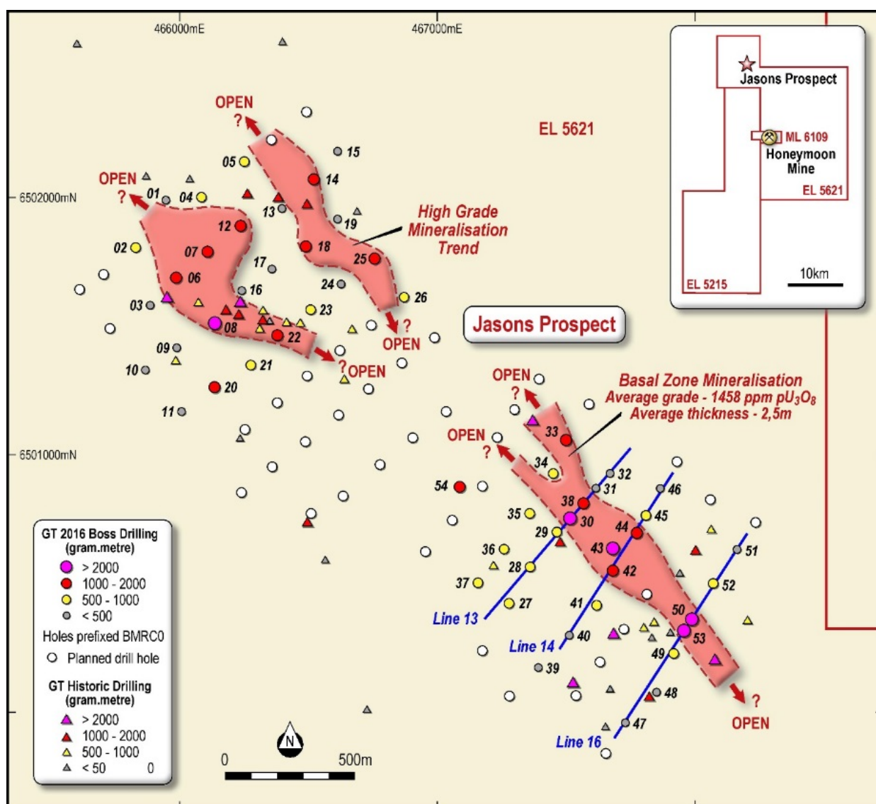
Figure 1: Location of drilling at the Jasons Prospect, approximately 15km north of the Honeymoon Mine site. Maximum grade times thickness (eU 3 O 8 [in ppm] x m) shown to assist in illustrating high-grade trends.
