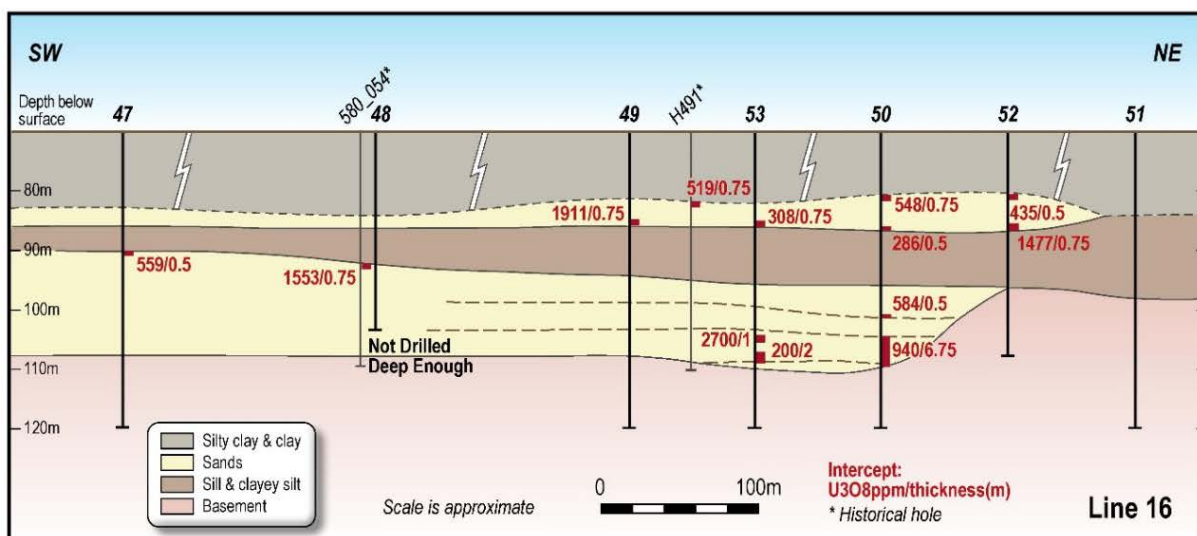
Figure 2: Example cross sections through Lines 13, 14 and 16. Results are shown as grade (ppm \text{eU}_3\text{O}_8 or \text{pU}_3\text{O}_8 / thickness in metres where available). Note: sections only show the bottom ~60m of each section.
