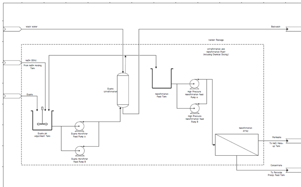
Figure 1: Neutralisation, Ultrafiltration & Nano-Filtration Flow Diagram
