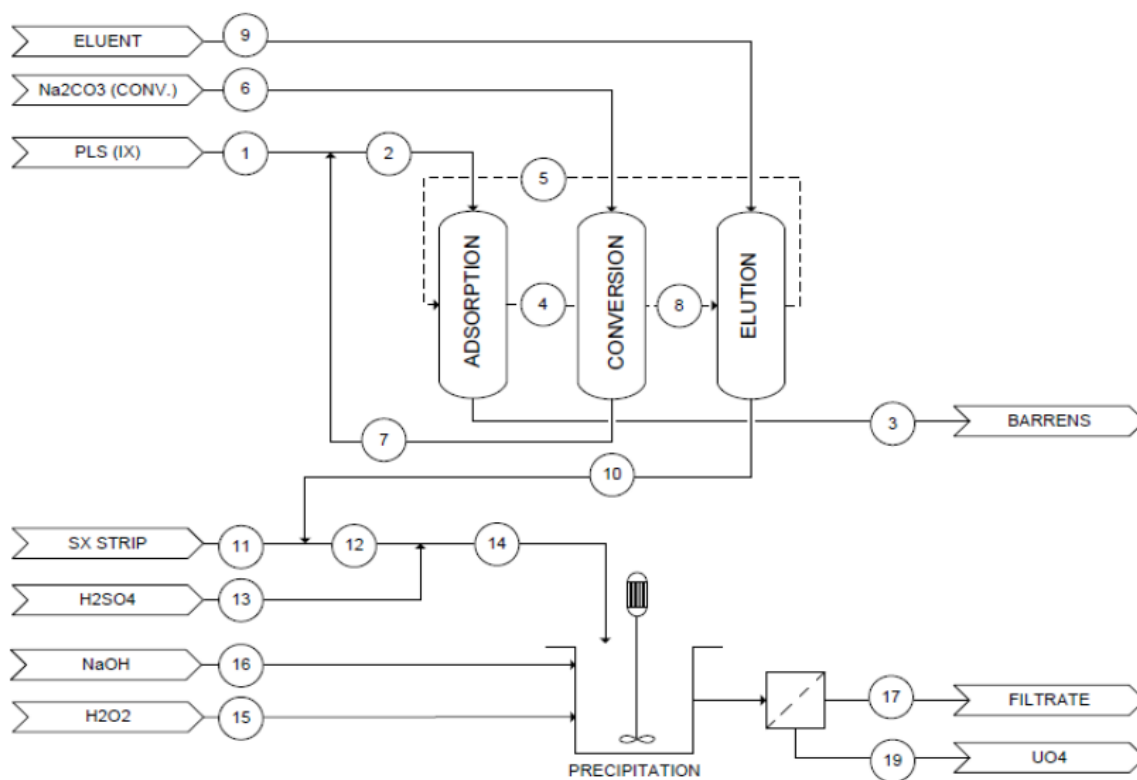
Figure 2: Two-Stage Elution Flow Diagram
