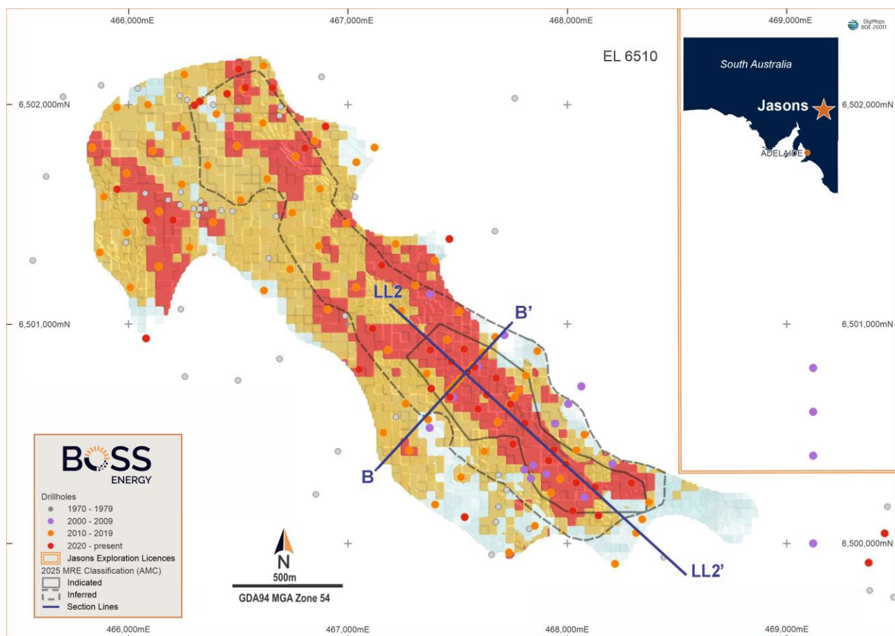
Figure 4: Jason's Deposit AMC 2025 block model and resource classification.
