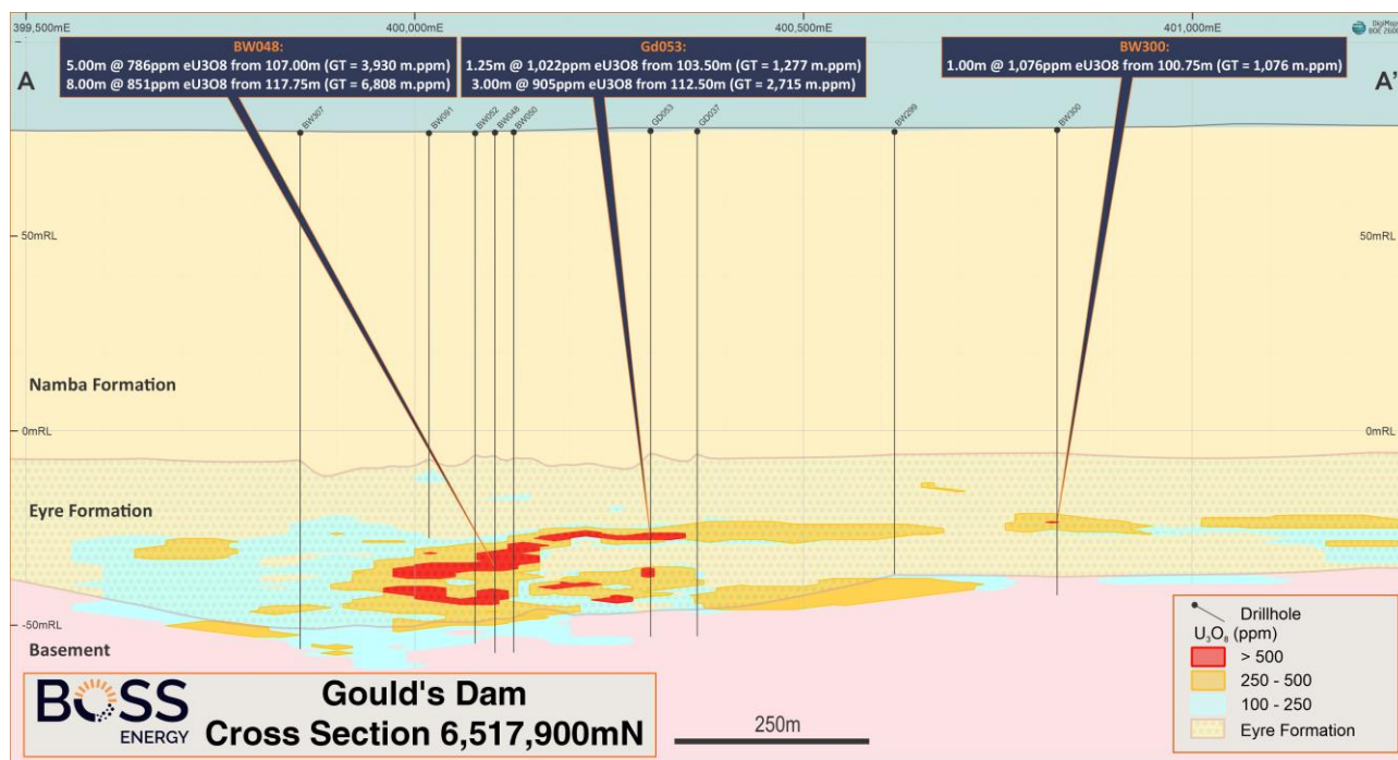
Figure 5: Gould's Dam cross section 6,517,900mN.
