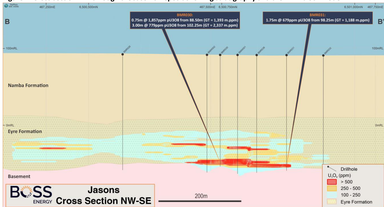
Figure 7: Cross section A-A through the Jason's Deposit showing stratigraphy and the MRE block model.
