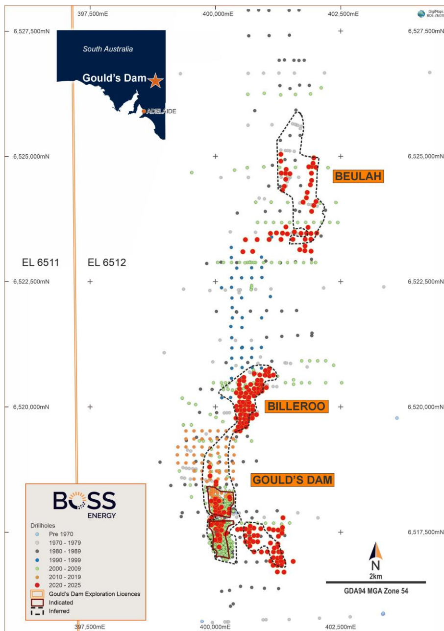
Figure 3: Gould's Dam map showing the various drilling campaigns and drill density.
