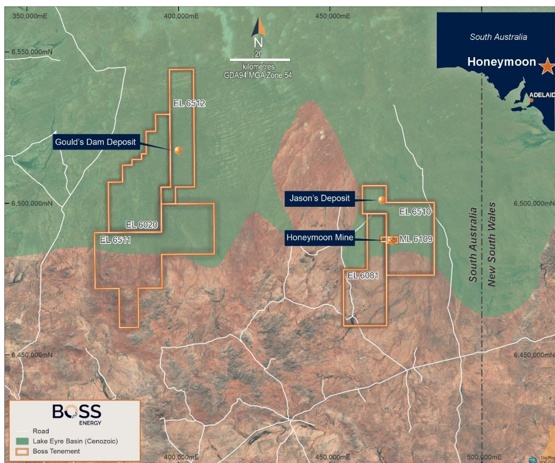
Figure 1: Location map showing the Honeymoon Mine relative to the Gould's Dam and Jason's Deposit.
