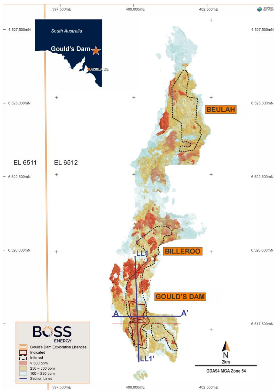
Figure 2: Gould’s Dam Deposit showing the amalgamation of Gould’s Dam prospect to the South, Billeroo prospect central, and Beulah prospect to the North, with continuous mineralisation over 15km strike length.
