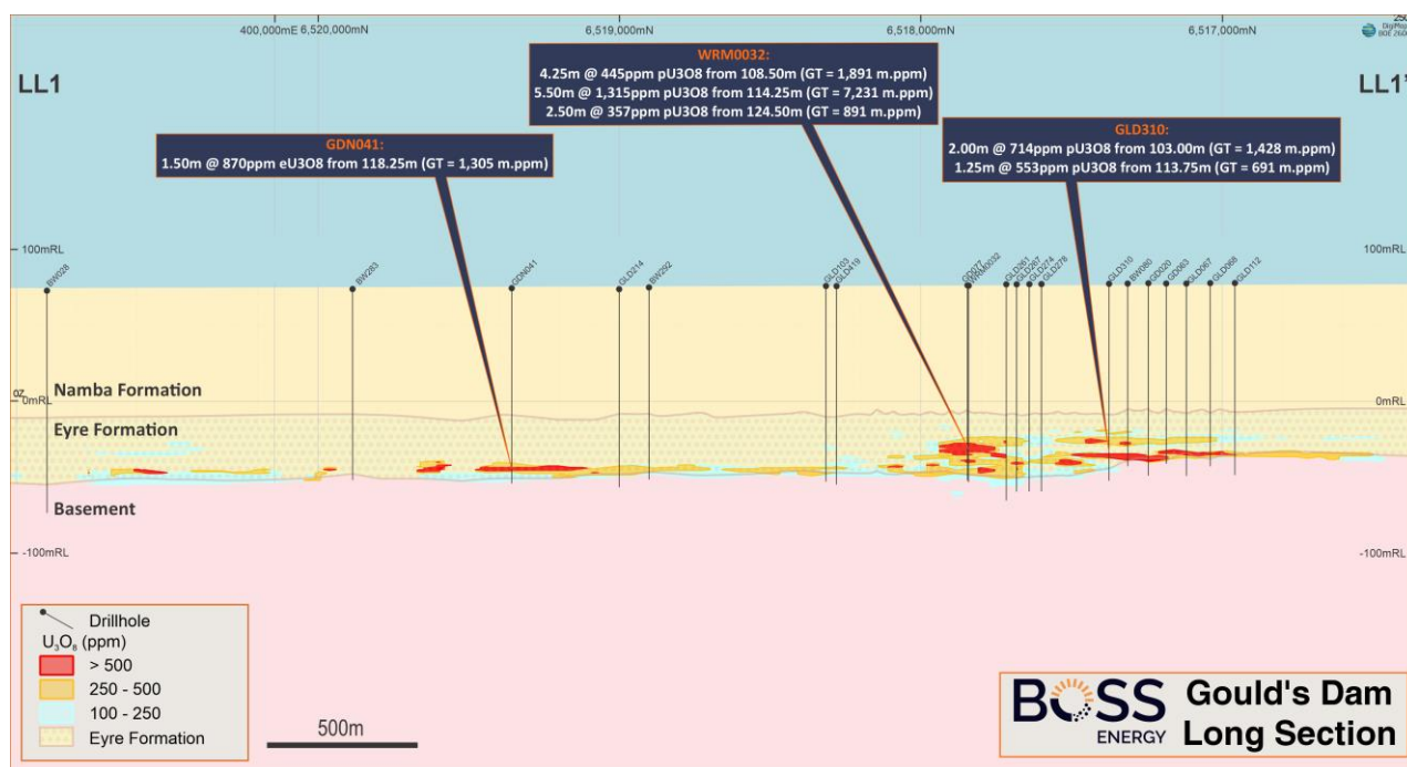
Figure 6: Gould's Dam long section. Mineralisation is predominantly located on the basal horizon, especially to the north. Five times vertical exaggeration this and subsequent sections.
