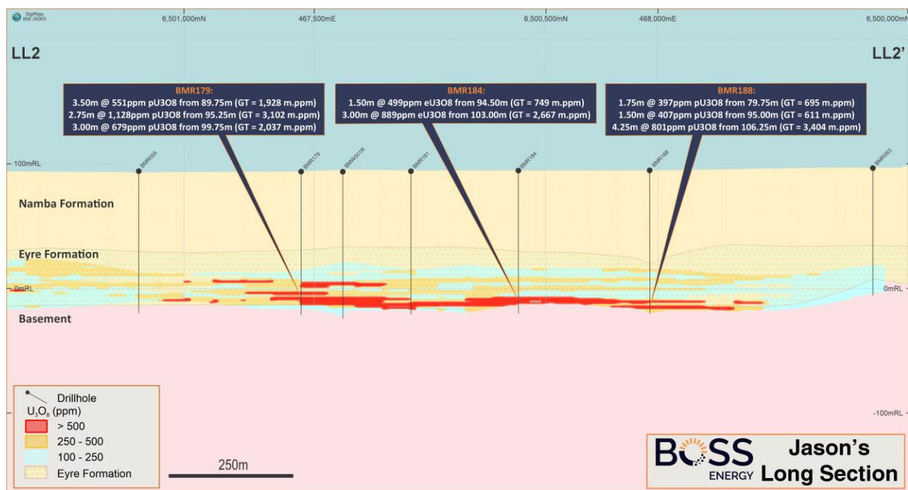
Figure 8: Long section through the Jason's Deposit showing the multiple mineralised horizons. The main horizon is the basal sequence.
