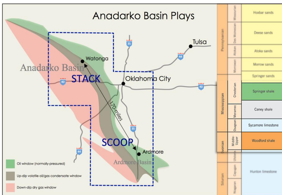
Figure 1. Anadarko Basin Plays
